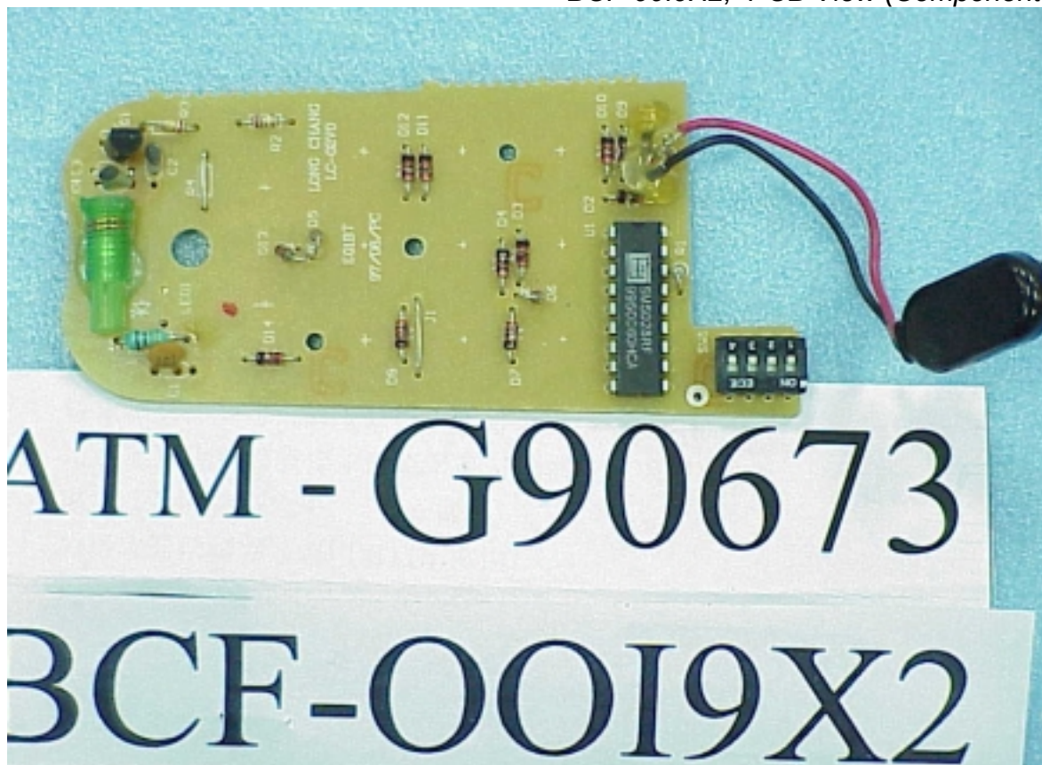
BCF-00I9X2, PCB View (Component Side)
