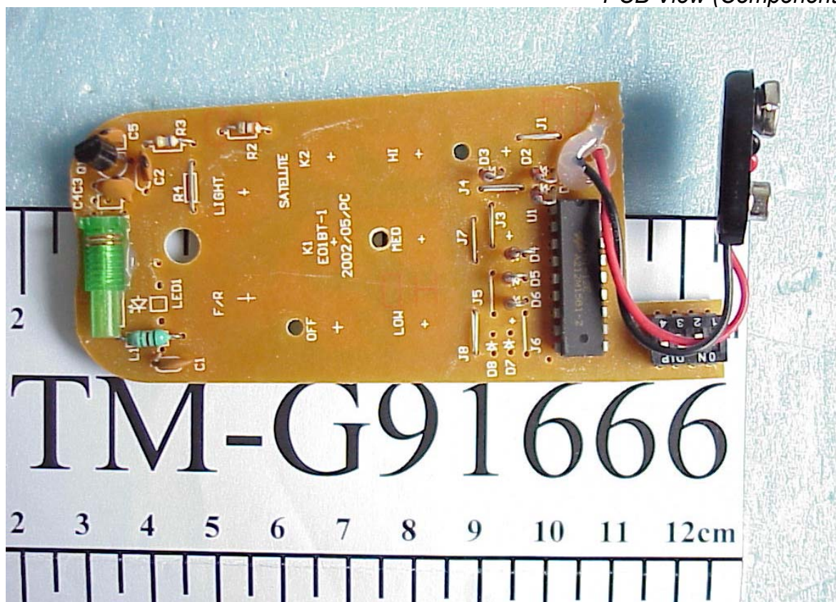
Photos 5 PCB View (Component Side)
