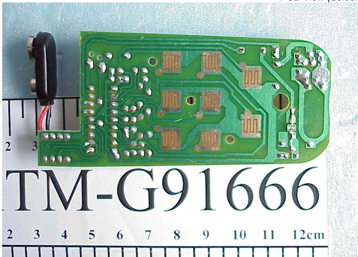
Photos 4 PCB View (Solder Side)
