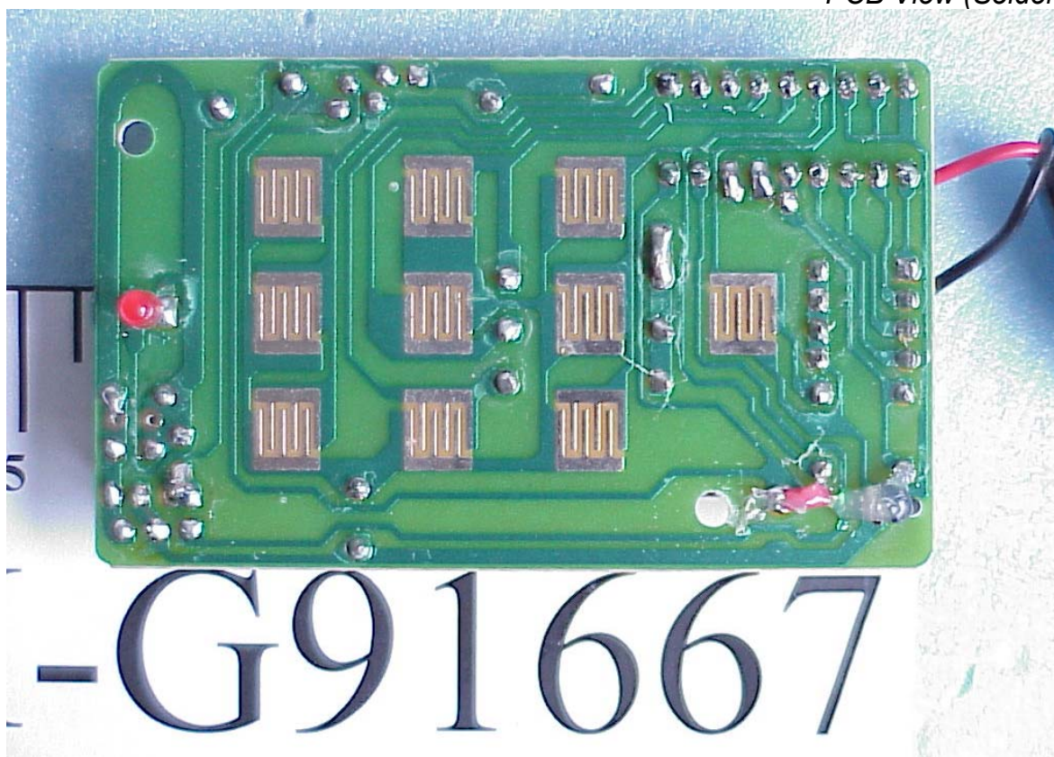
Photos 5 PCB View (Solder Side)
