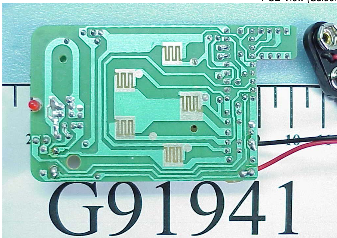
Photos 5 PCB View (Solder Side)
