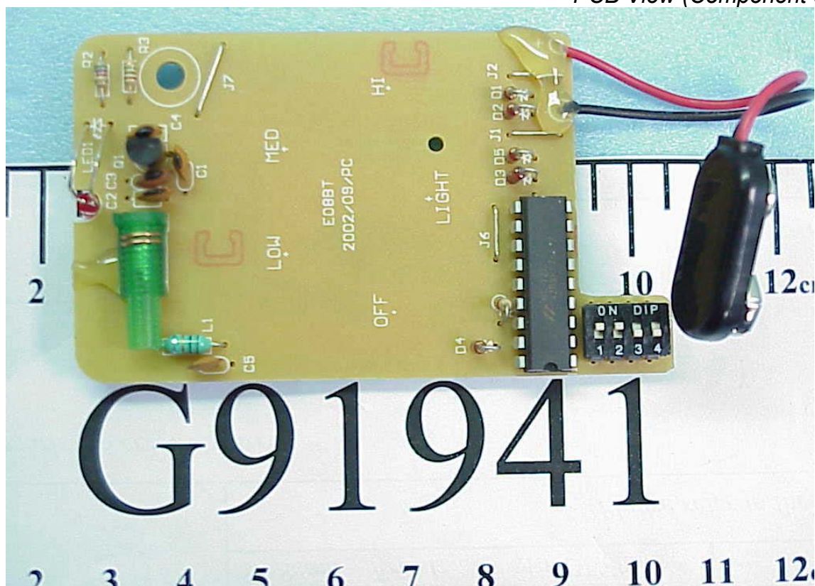
Photos 4 PCB View (Component Side)
