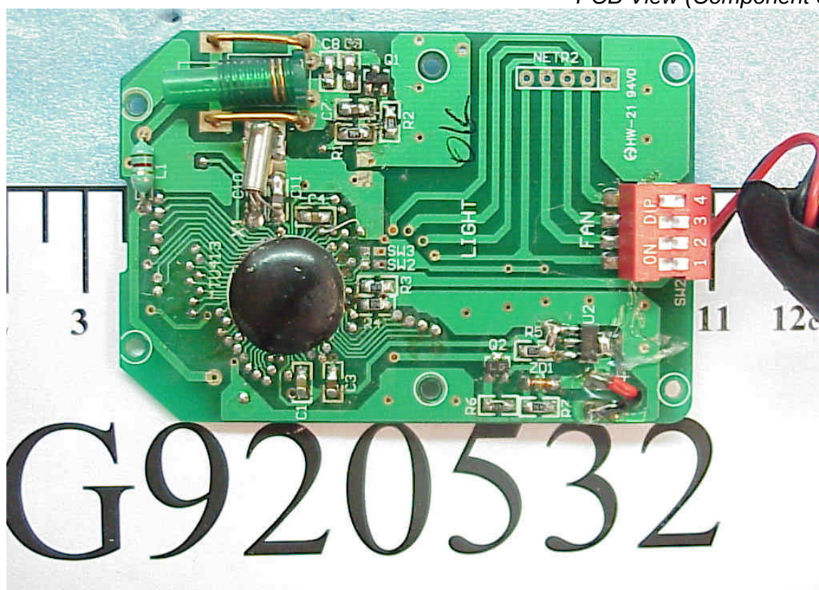
PCB View (Component Side)
