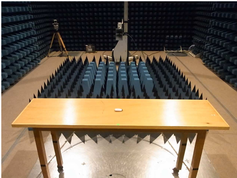
Rear View (1GHz – 3.15GHz)
