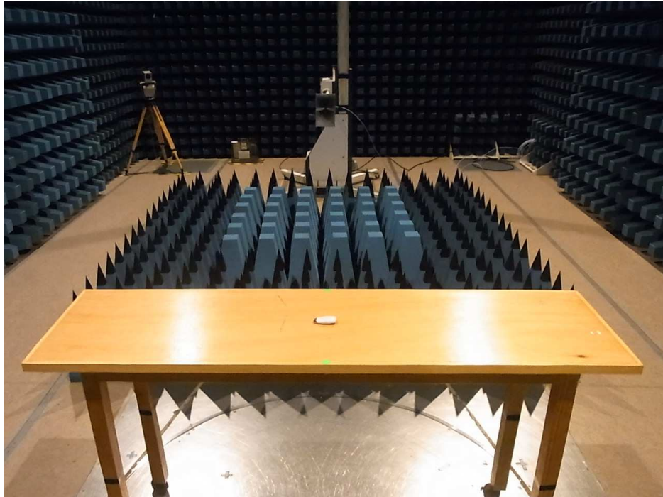
Front View (1GHz – 3.15GHz)
