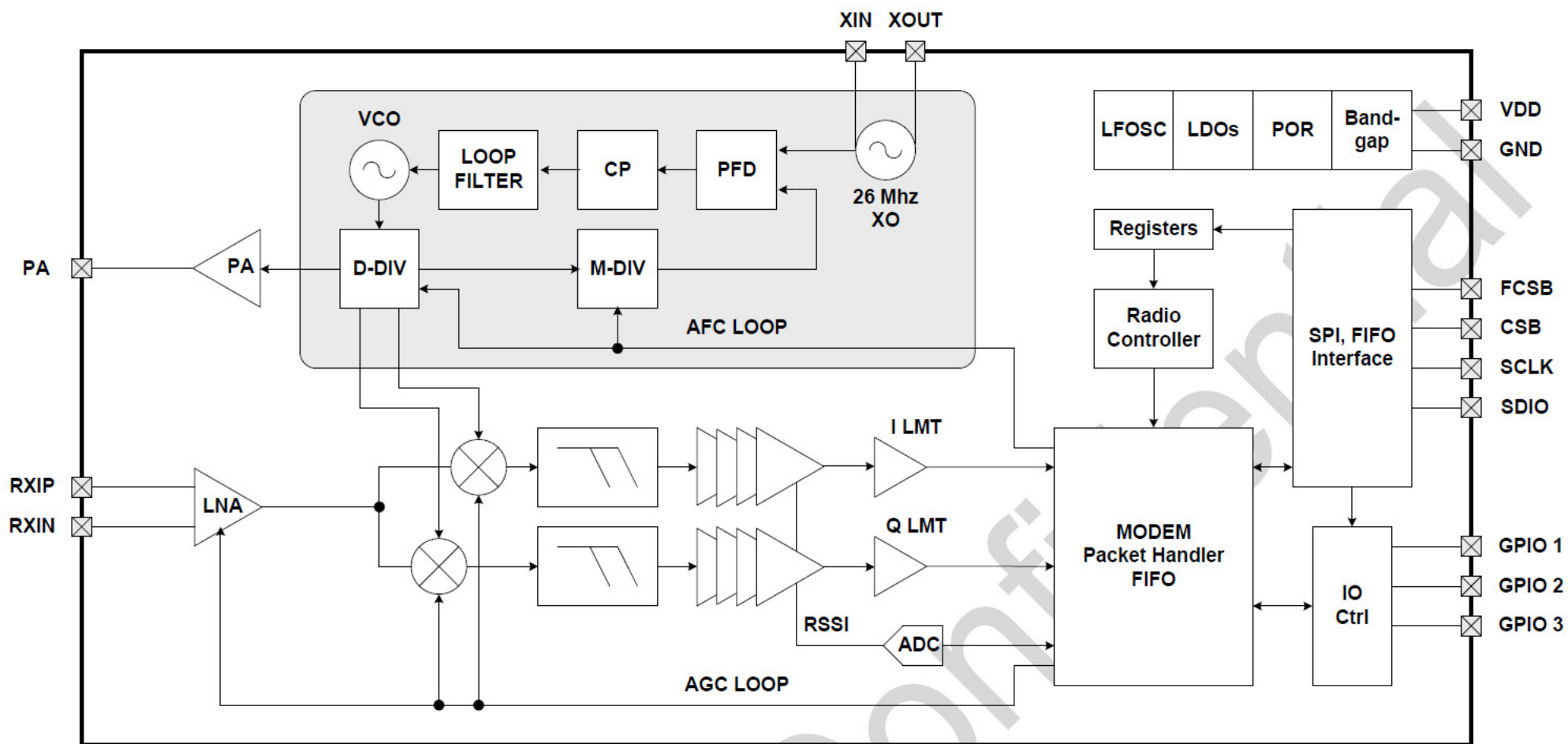
Figure 4. Functional Block Diagram
