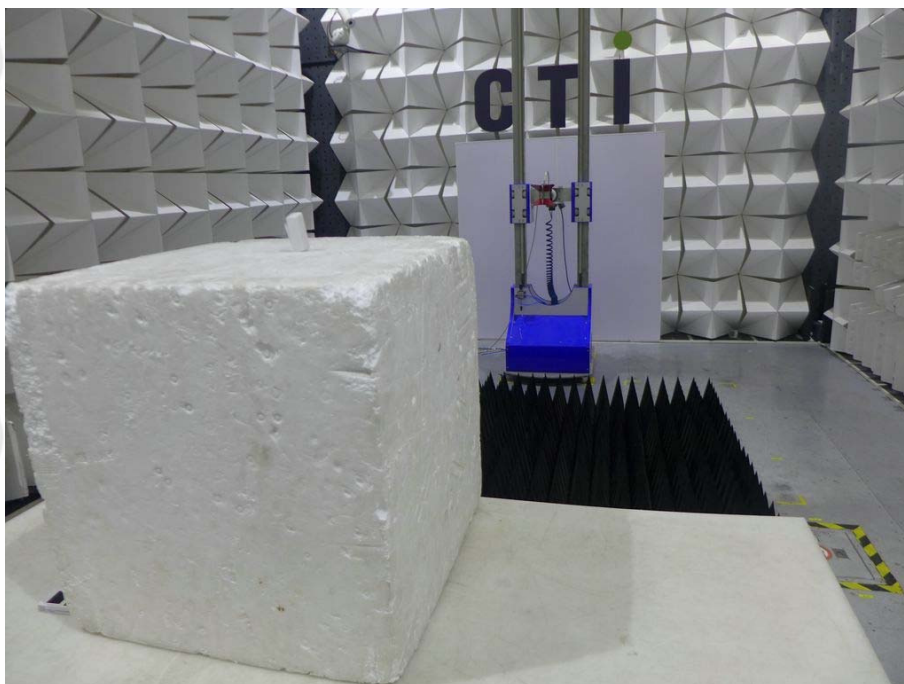
Radiated spurious emission Test Setup-4 for WD-MT2(Above 1GHz)
