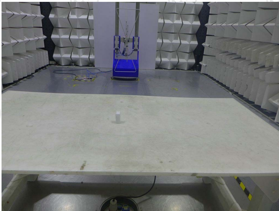
Radiated emission Test Setup-1 for GS-MT2(30MHz~1GHz)
