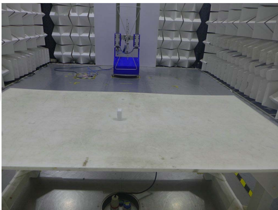
Radiated emission Test Setup-2 for WD-MT2(30MHz~1GHz)
