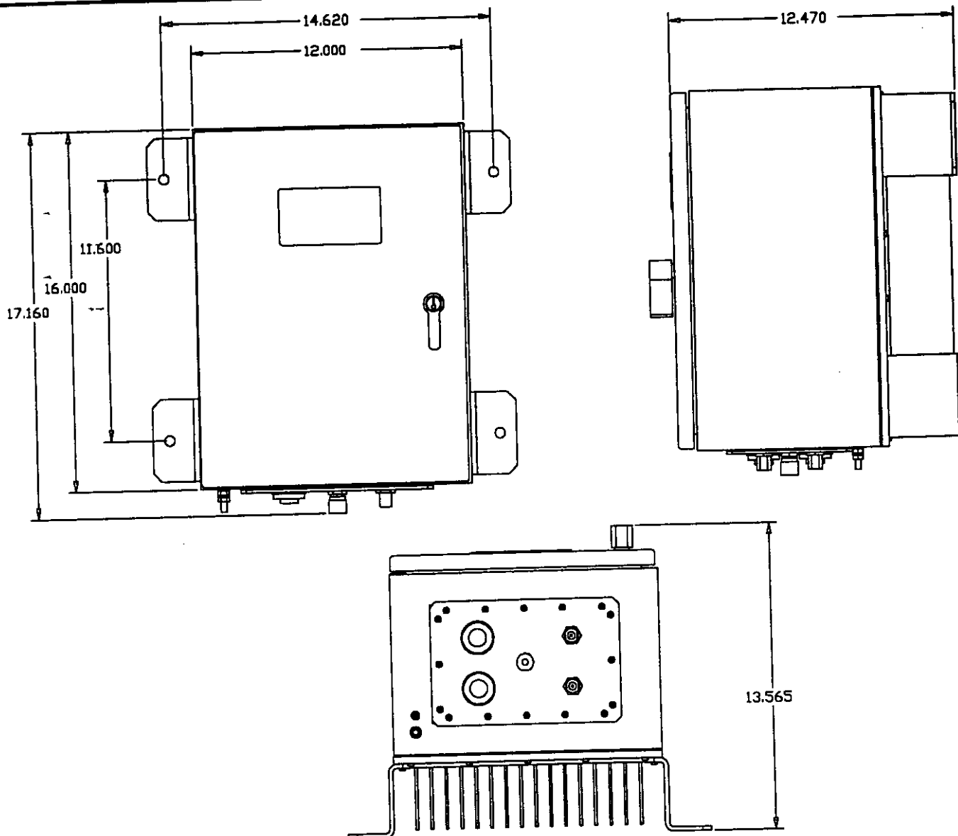
Figure 1-1 SelectAmp 1800 Outline Drawing
