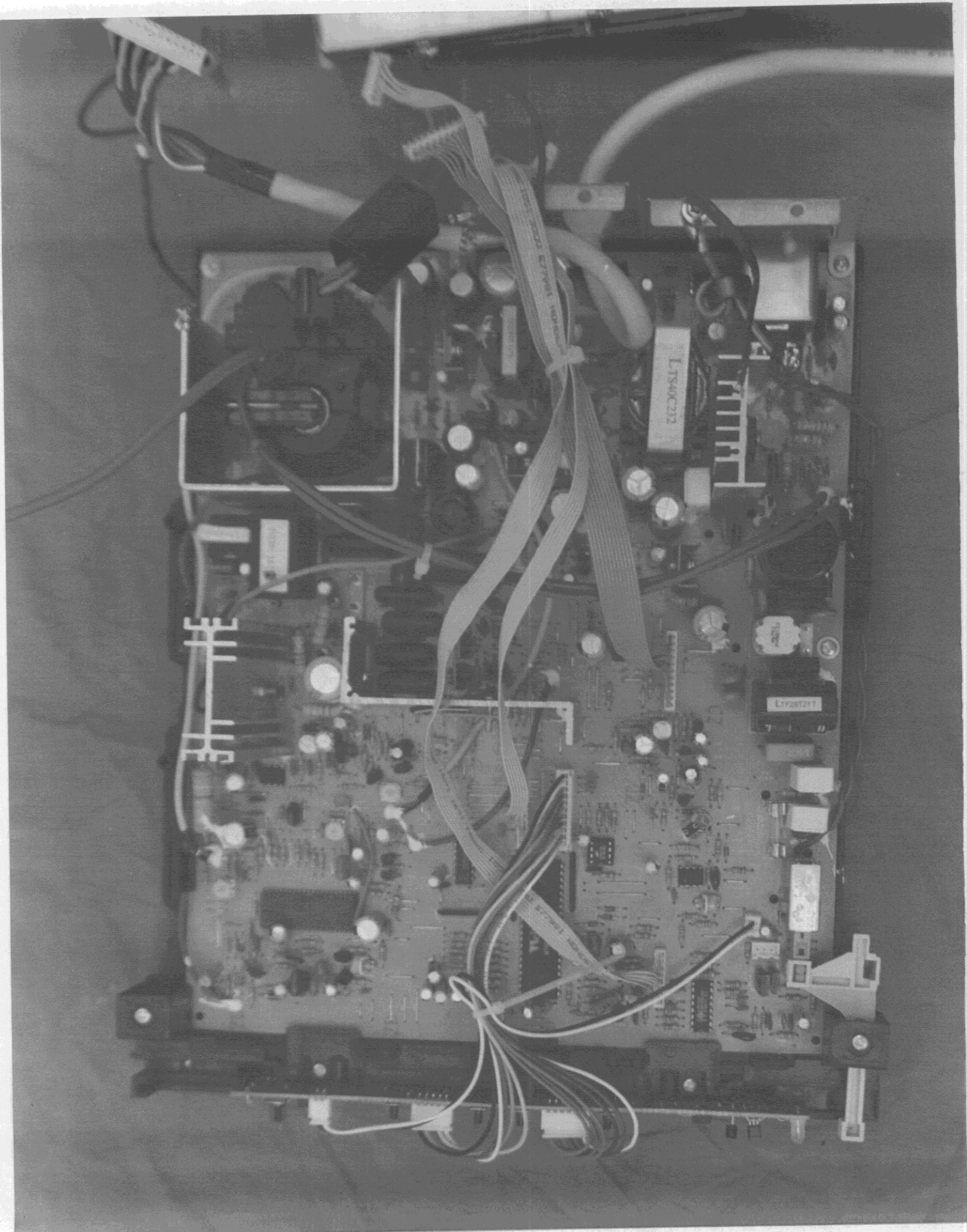
Figure 6 Main PCB Board, Component Side
