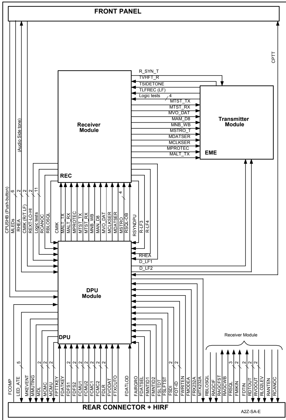
Figure 8 - Signal Connections
