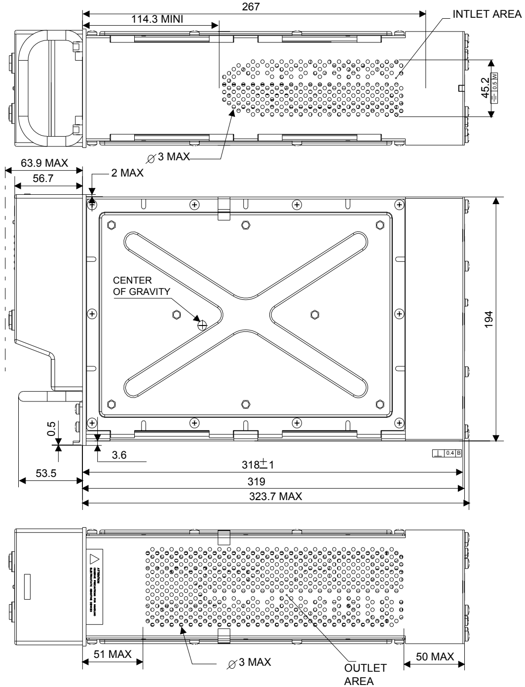
Figure 5 – Dimensions
