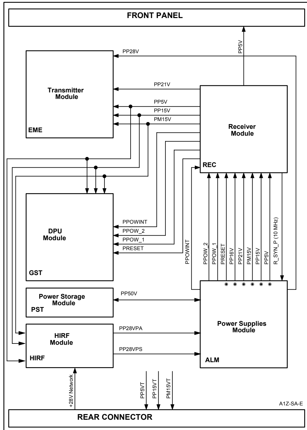
Figure 7 - Power Supply Connections
