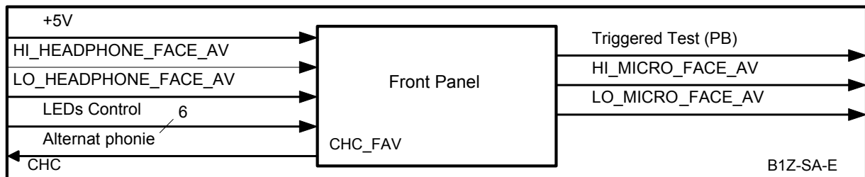
Figure 9 - Wired Chassis (CHC) Block Diagram
