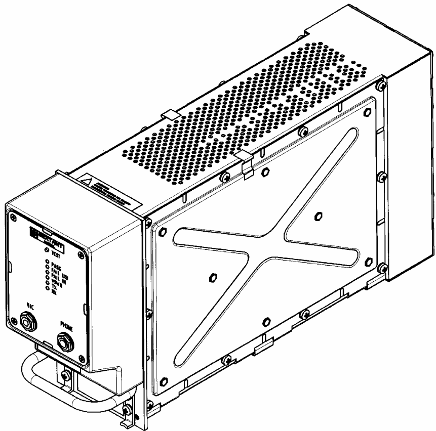
Figure 1 - EVR716/750 Unit
