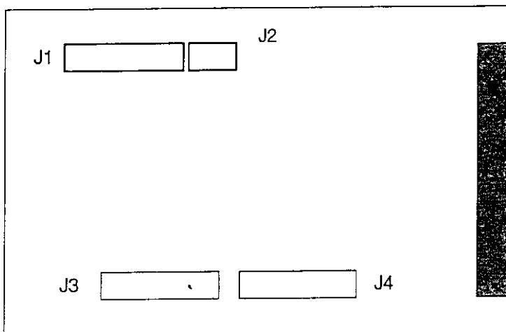
Figure 3-2 : Connector locations for SPI module - new board
