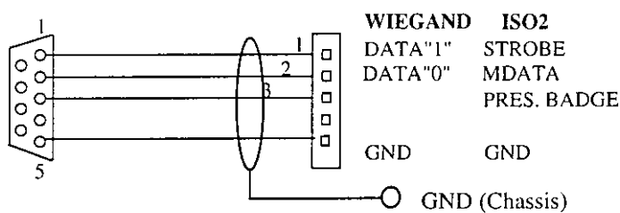
Wiring diagram
