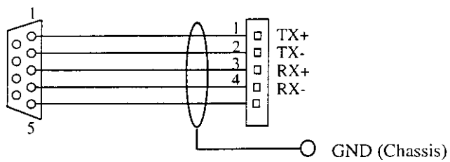
Wiring diagram
