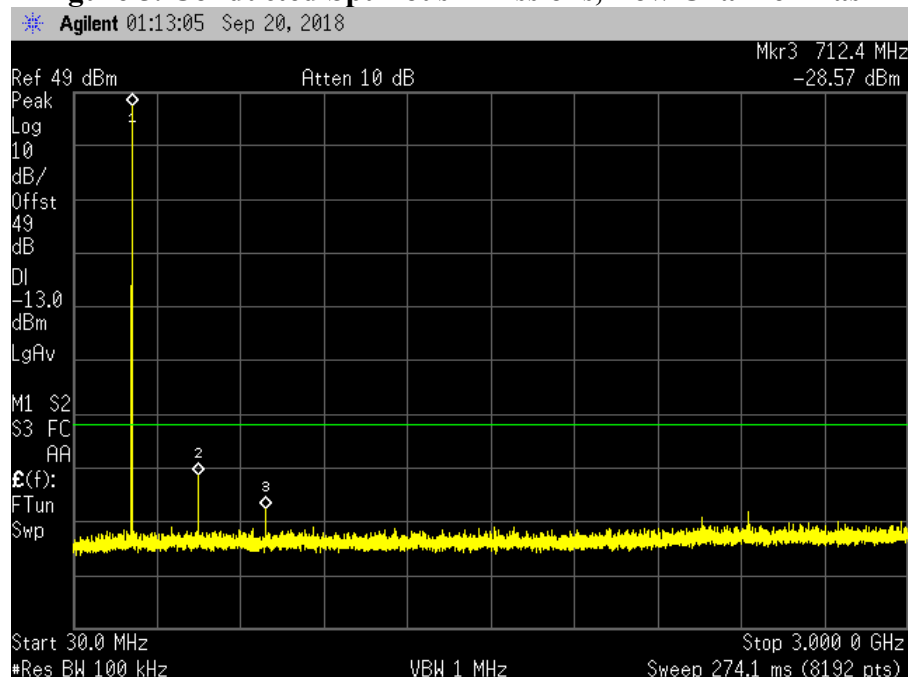
Figure 5. Conducted Spurious Emissions, Low Channel Mask
