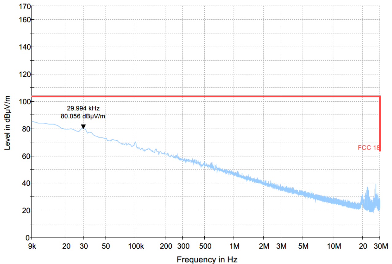
Plot # 1 Unwanted Emissions: 9 kHz - 30 MHz
