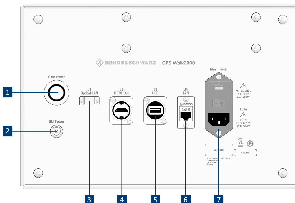
Figure 4-1: Gate controls and connectors
