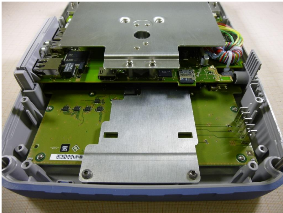
Photo 3: Bottom view
