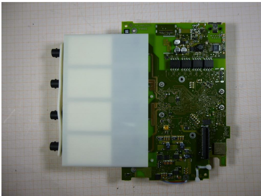
Photo 8: PCB top view
