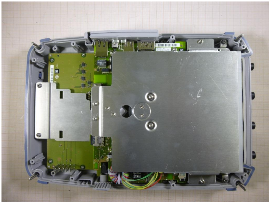
Photo 1: Back cover removed
