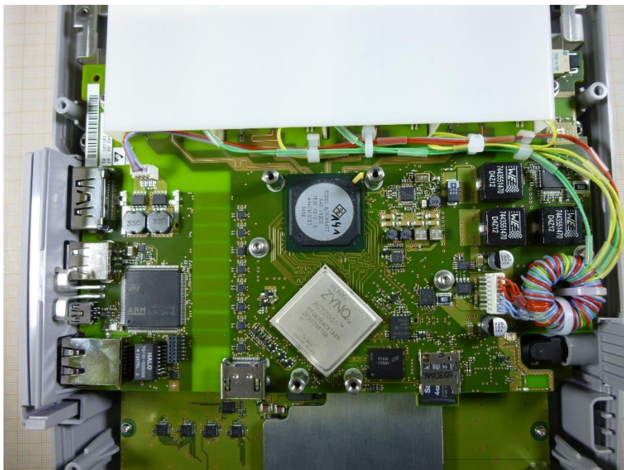
Photo 6: PCB
