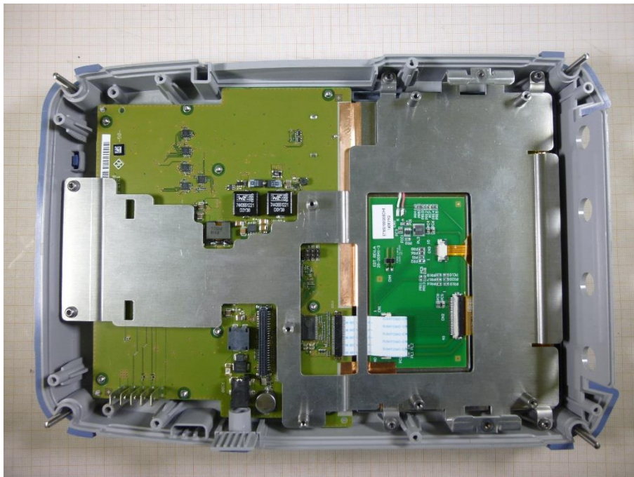
Photo 7: PCB removed
