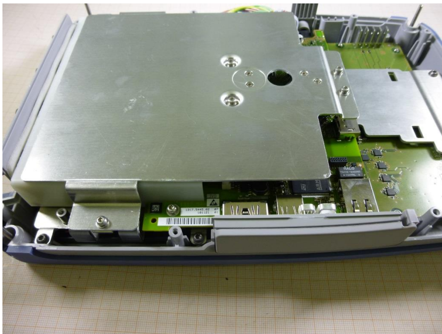
Photo 4: Connector side
