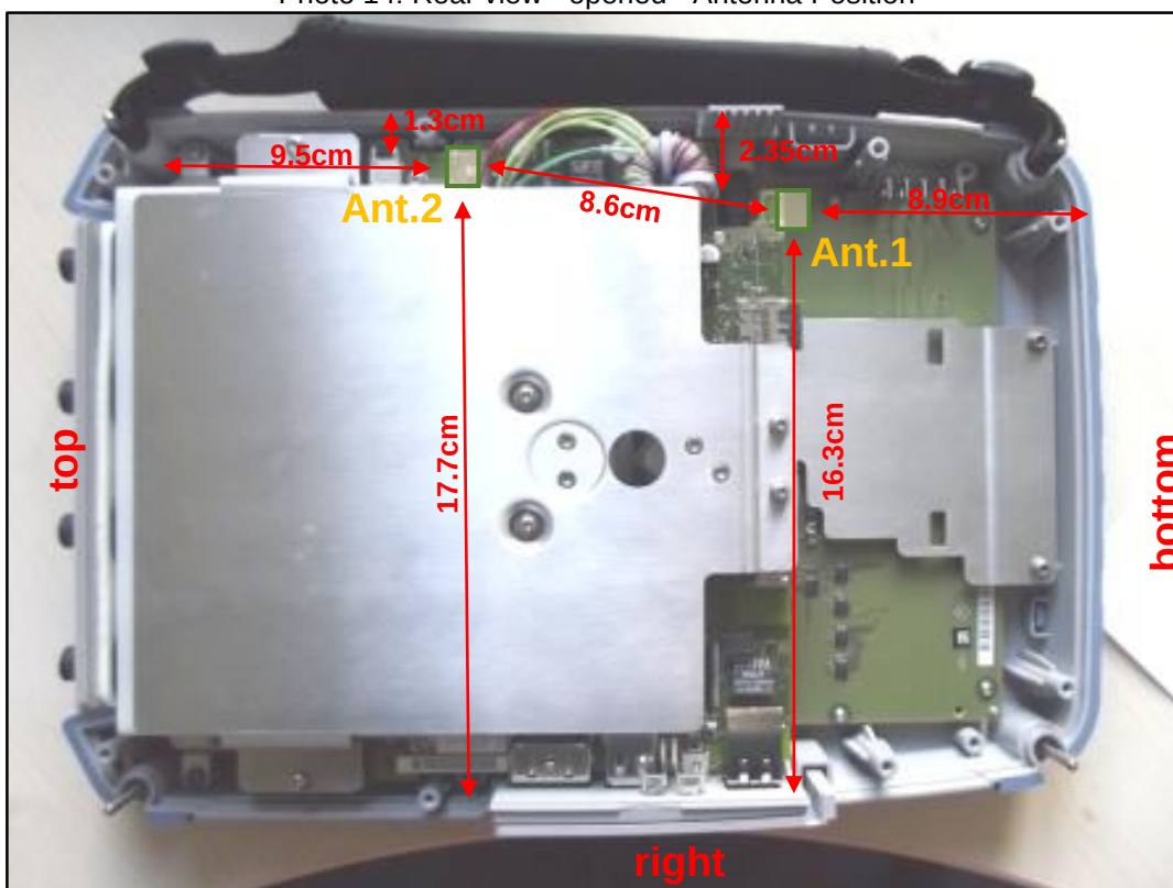
Photo 14: Rear view - opened - Antenna Position
