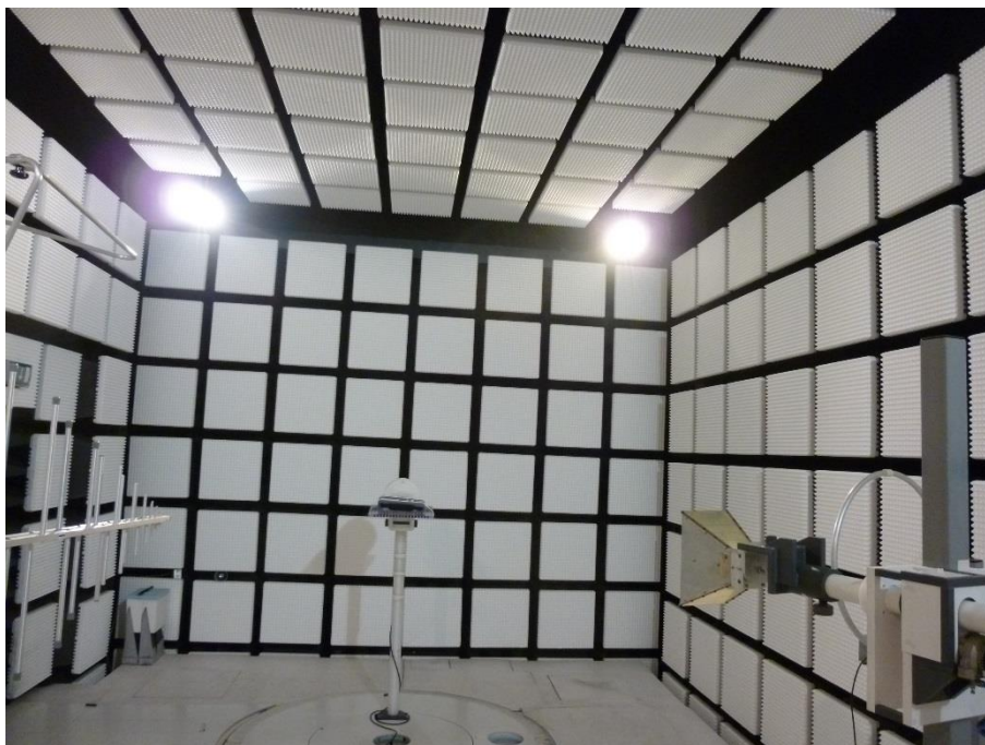
Photo 8: Fully anechoic chamber
