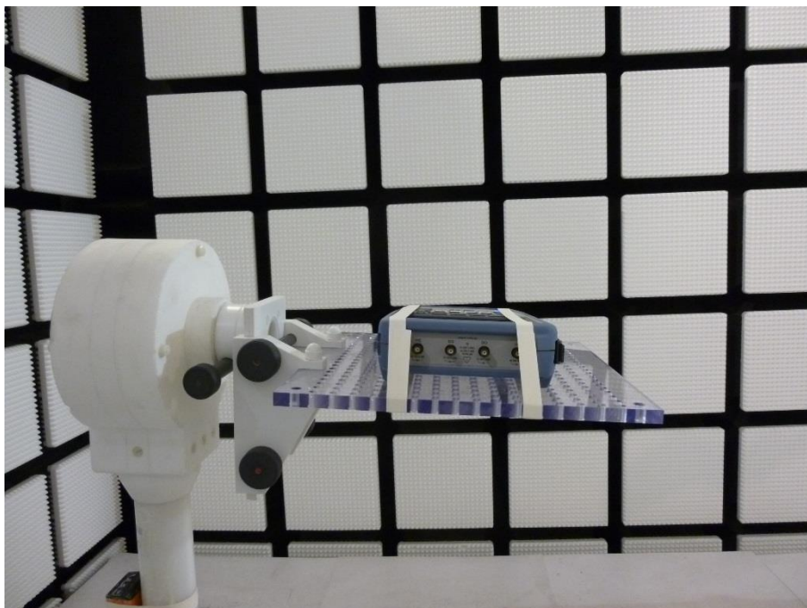
Photo 4: Fully anechoic chamber
