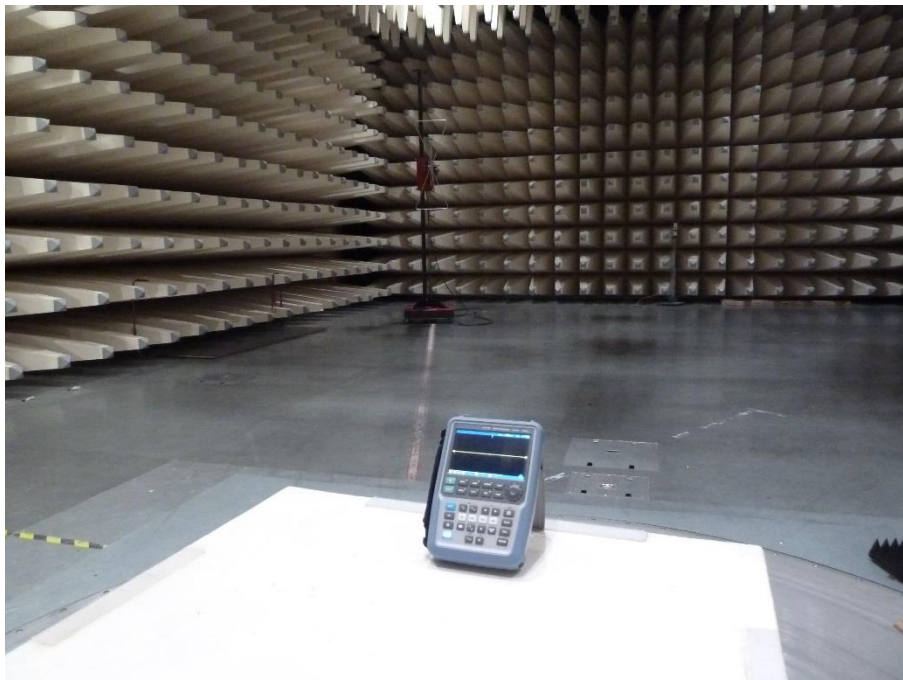
Photo 1: Semi anechoic chamber
