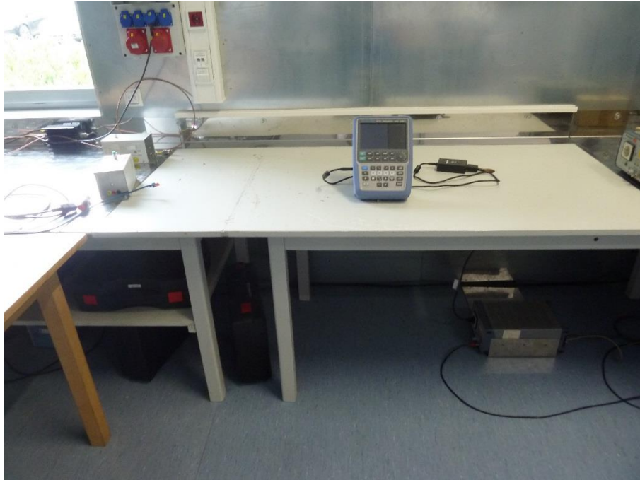
Photo 9: AC conducted measurement
