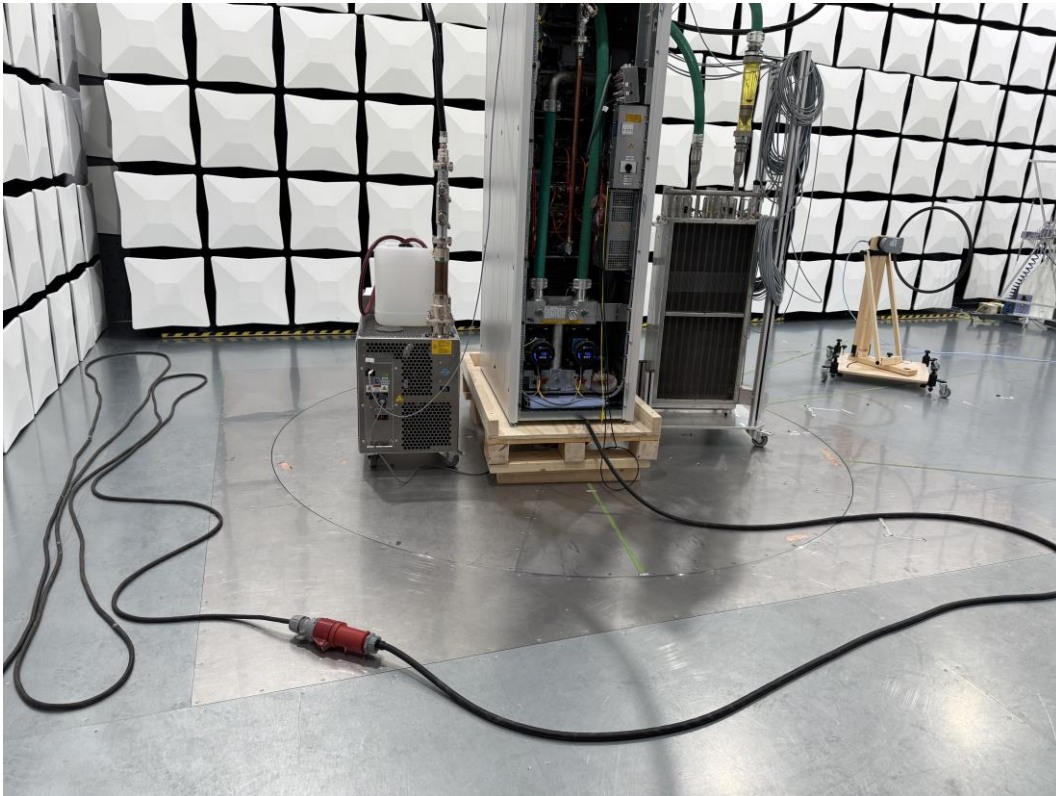
Photograph 5: Overall view. Radiated cabinet measurement with signal power on EUT 5 kW. The door of the chamber is open to get the power supply cable in the chamber.
