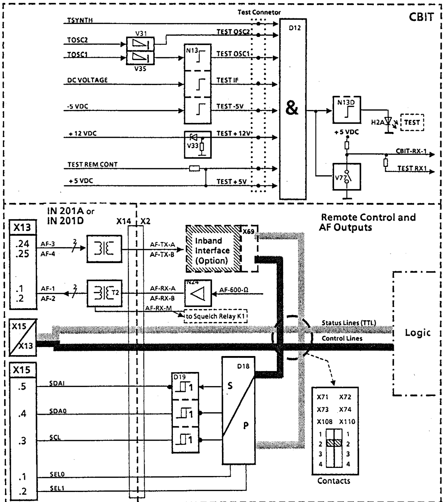
Fig. 5.2 VHF Rx Unit EU 231, Block Diagram (Remote Control and CBIT)
