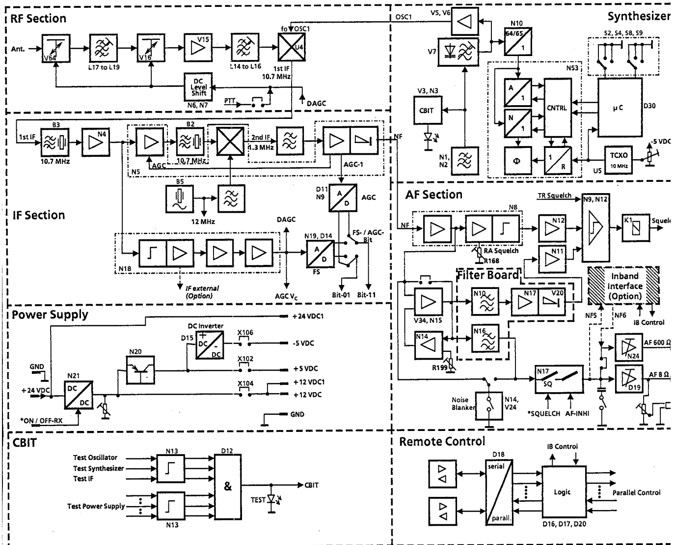
Fig. 5.1 VHF Rx Unit EU 231, Block Diagram (RF Section, Synthesizer, AF Section and Power Supply)
