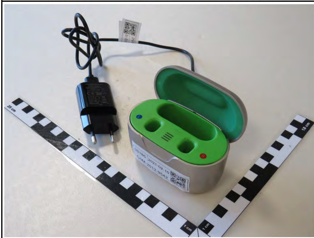
OPEN EUT WITH AC/DC-ADAPTOR IN PERSPECTIVE
