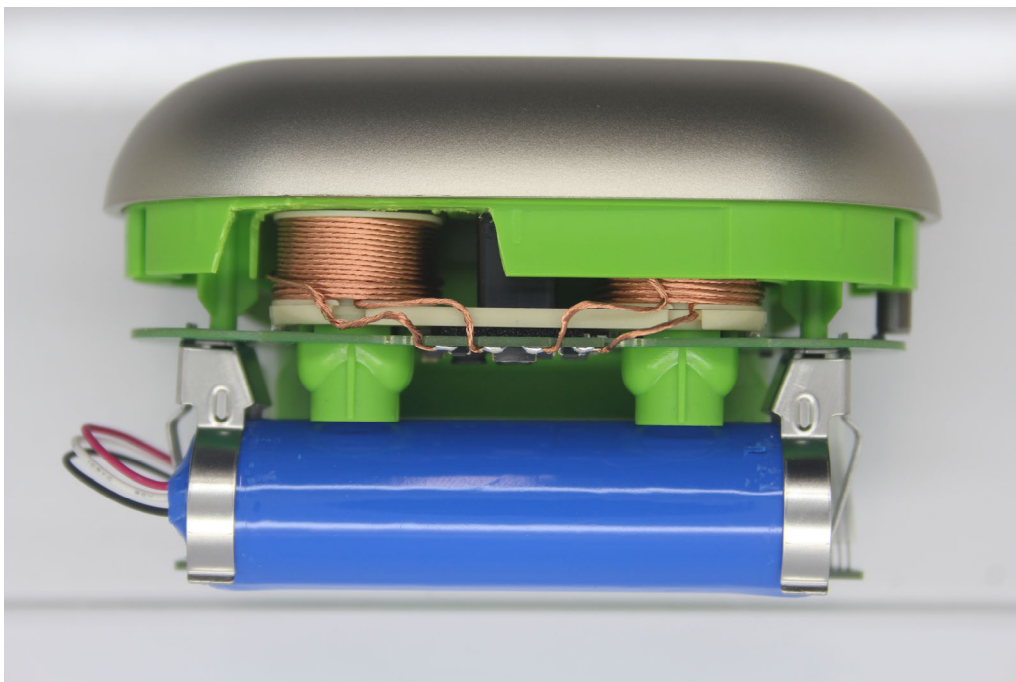
Detailed view of Coils –Cover Closed
