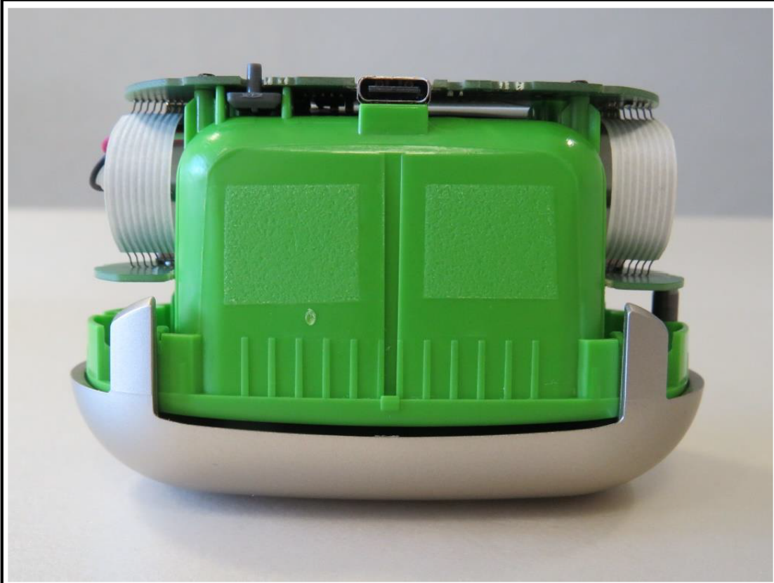
EUT WITHOUT COVER REAR SIDE
