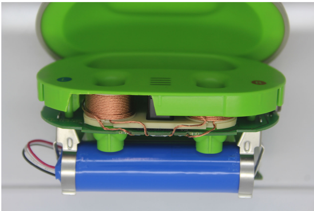
Detailed view of Coils –Cover opened
