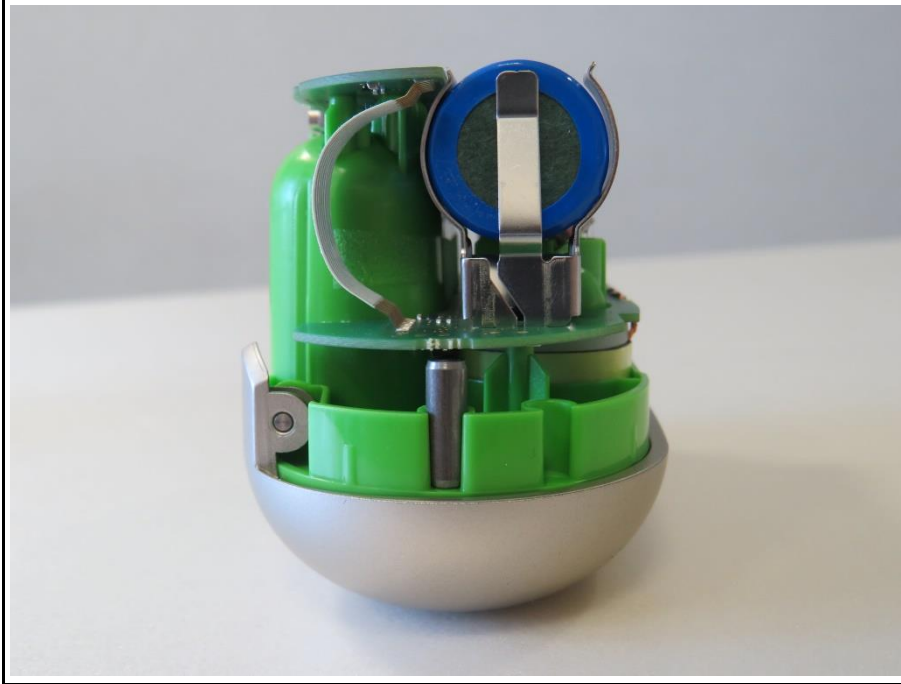
EUT WITHOUT COVER RIGHT SIDE
