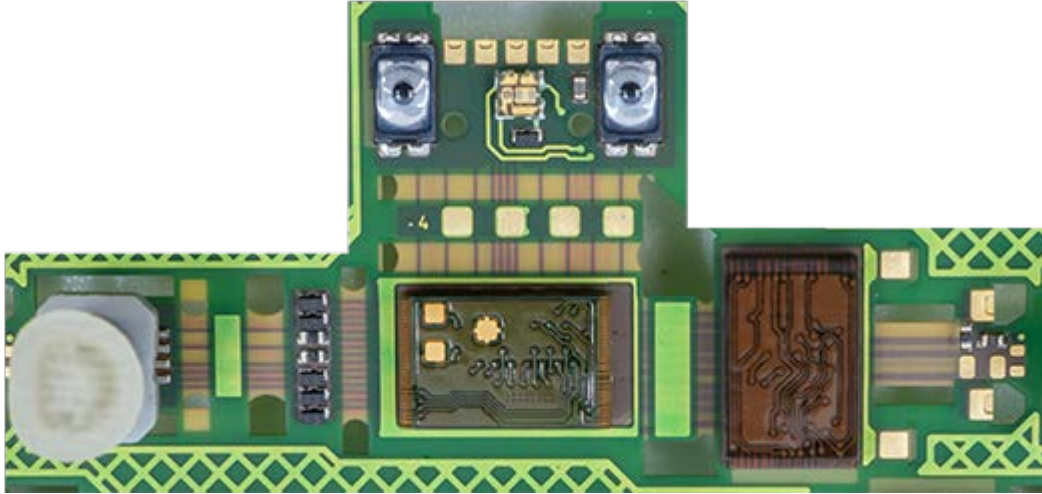
Bottom view
