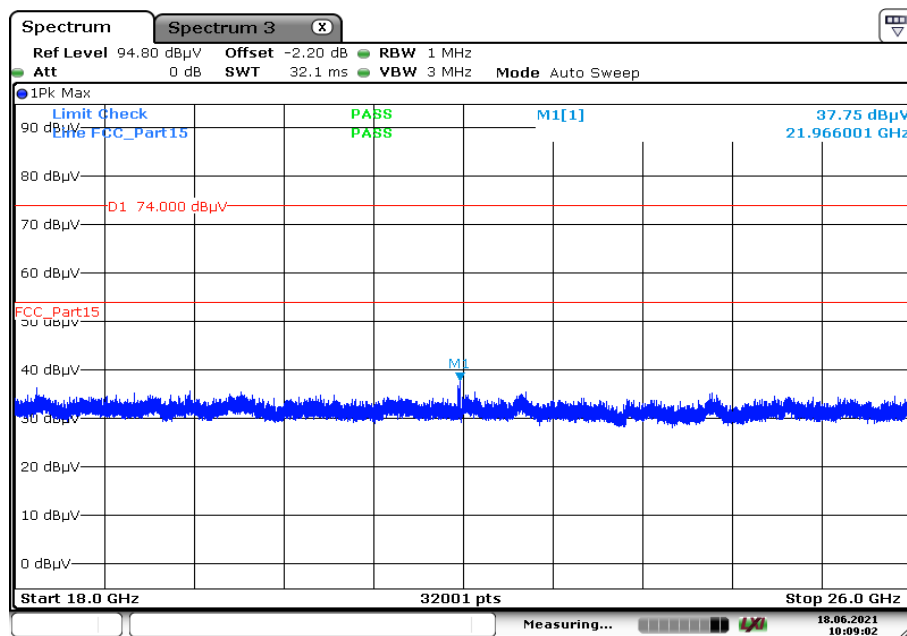
Plot 4: 18 GHz to 26 GHz, TX mode, mid channel, vertical & horizontal polarization
