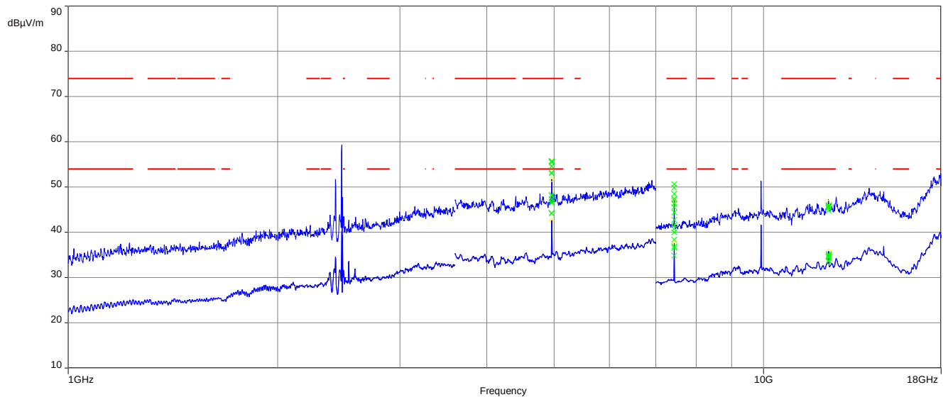
Plot 5: 1 GHz to 18 GHz, TX mode, high channel, vertical & horizontal polarization
