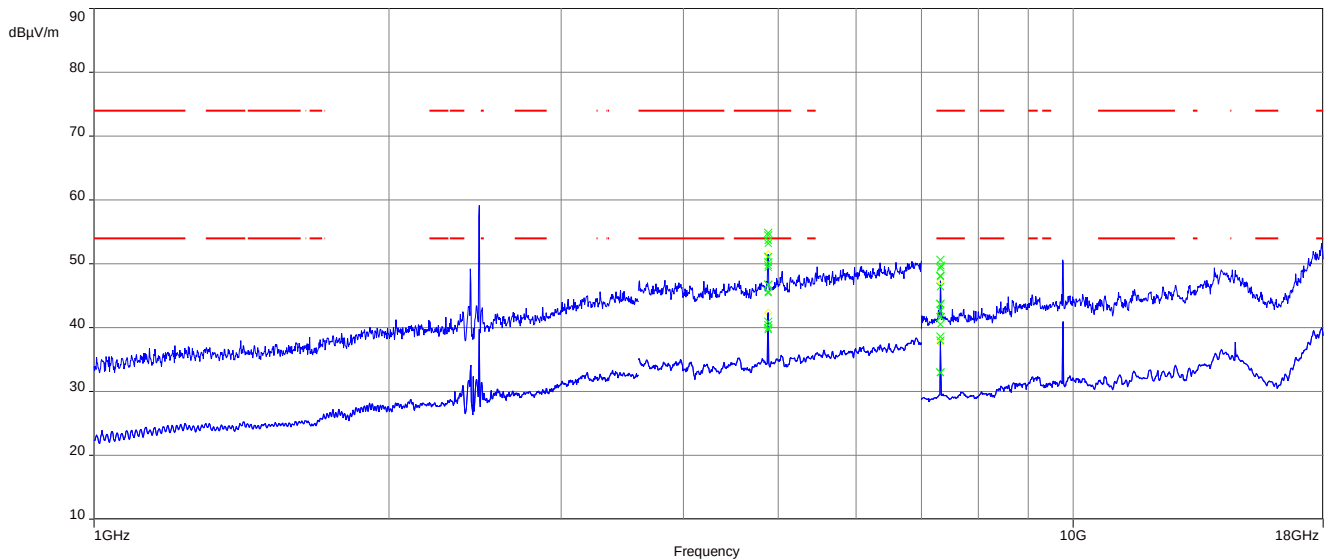
Plot 3: 1 GHz to 18 GHz, TX mode, mid channel, vertical & horizontal polarization
