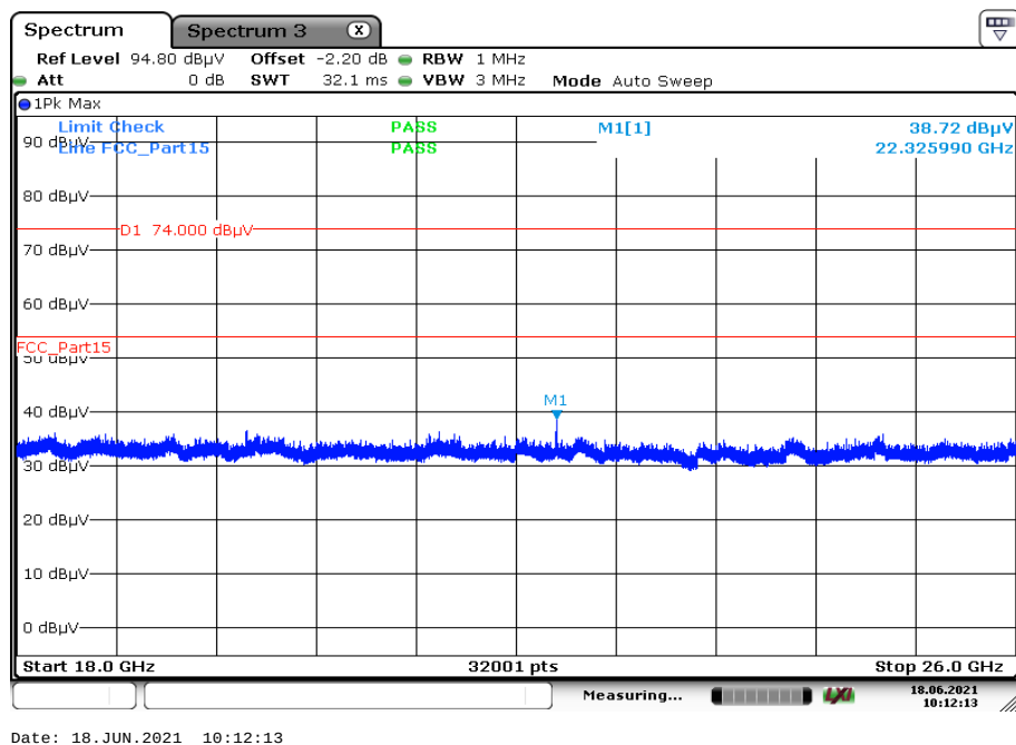
Plot 6: 18 GHz to 26 GHz, TX mode, high channel, vertical & horizontal polarization
