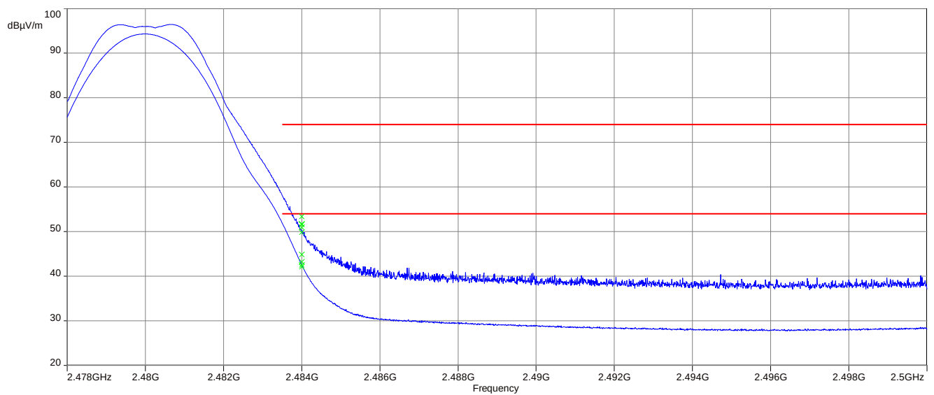
Plot 2: Upper band edge, vertical & horizontal polarization
