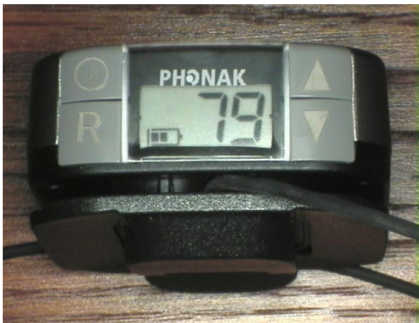
fig. 6 Campus S front view ON state, transmitting on channel 79 (channel 79 is a Phonak reference)
