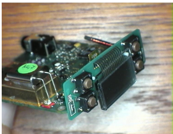
fig 3. Print upper side with LCD module
