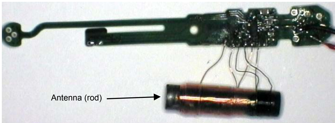
Figure 3 PCB bottom view
