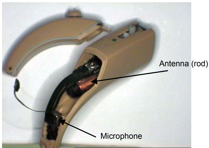
Figure 1 Internal view of the BICROS CTX
