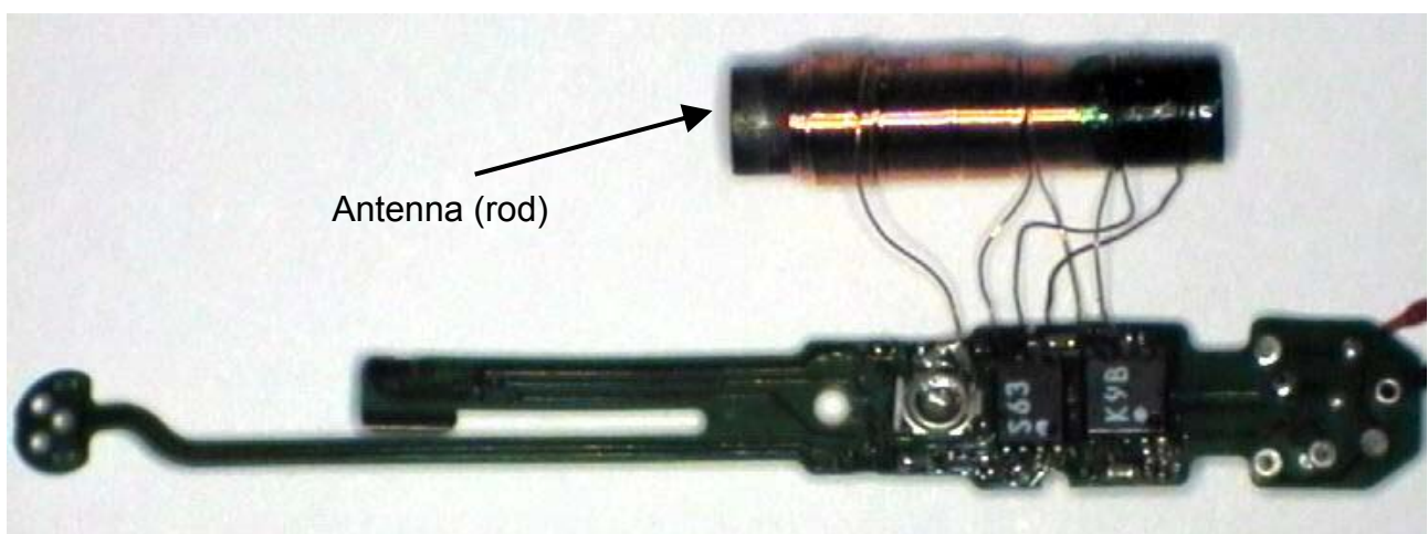
Figure 2 PCB top view
