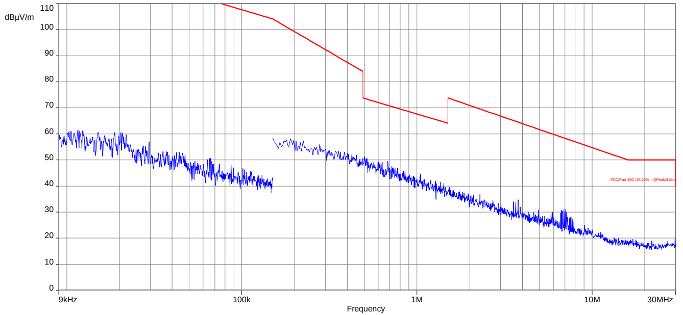
Plot 1: 9 kHz to 30 MHz, channel 00, transmit mode, unmodulated carrier
