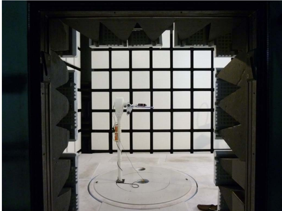
Photo 1: Anechoic chamber test setup
