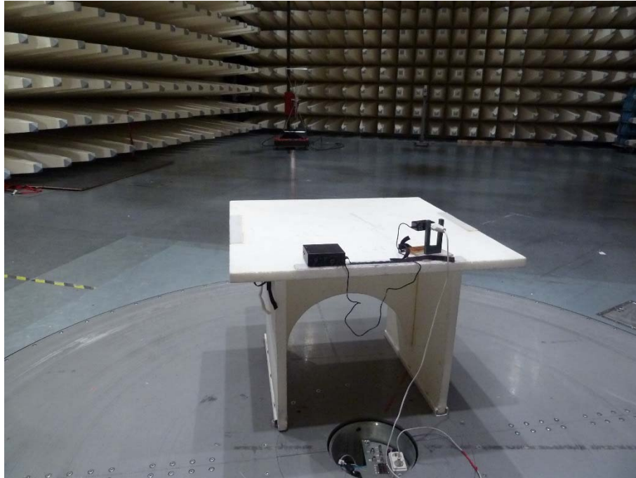
Photo 7: Semi-anechoic chamber test setup
