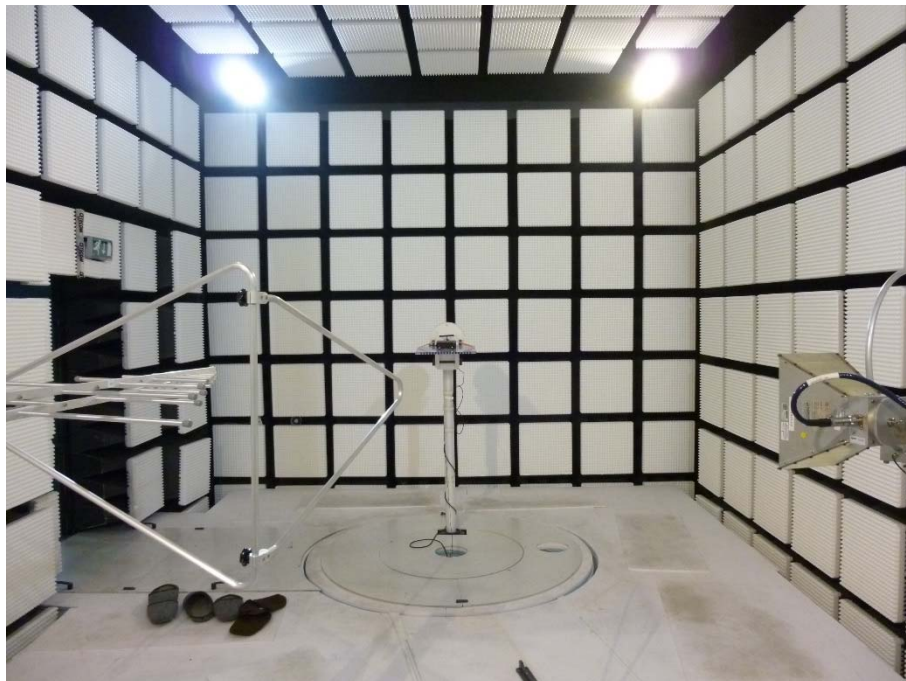
Photo 6: Anechoic chamber test setup
