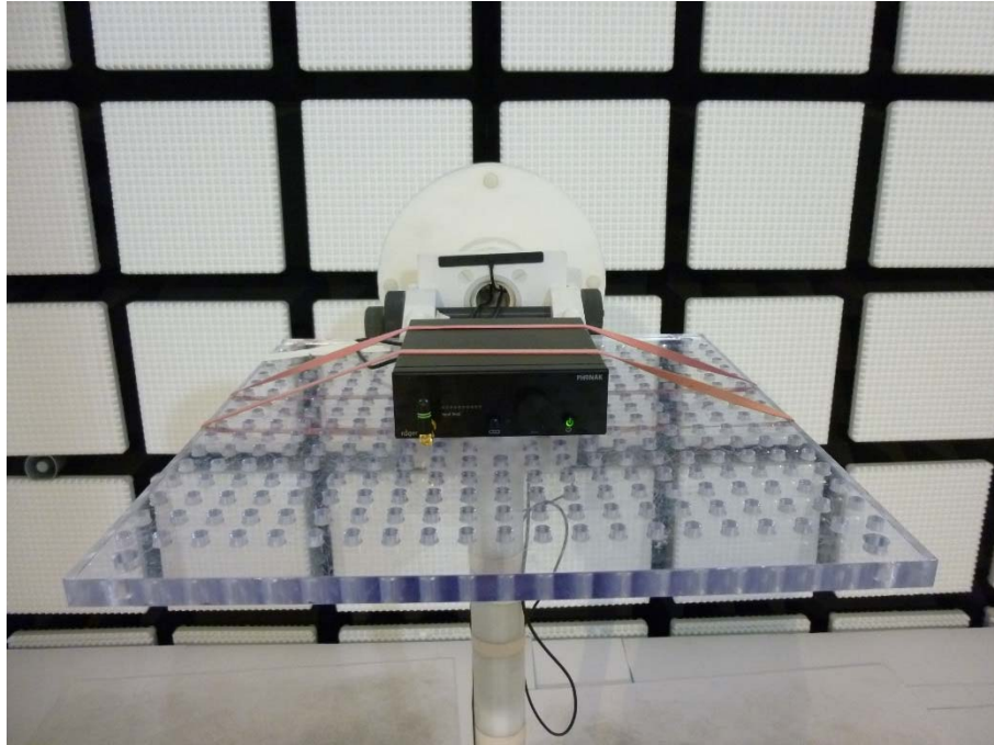
Photo 5: Anechoic chamber test setup
