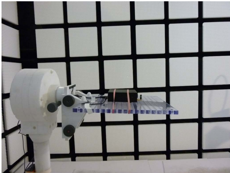
Photo 2: Anechoic chamber test setup
