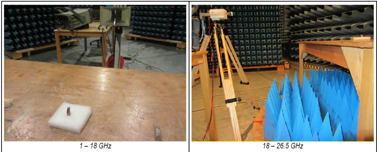
Fig 3 Spurious emissions – 1 GHz- 26.5 GHz
