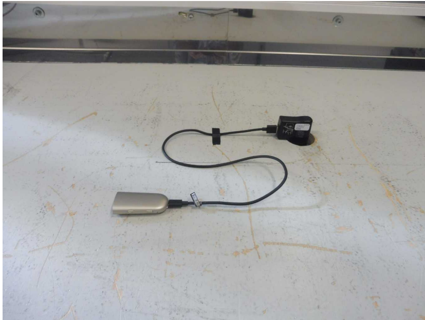
Photo 9: AC conducted test setup
