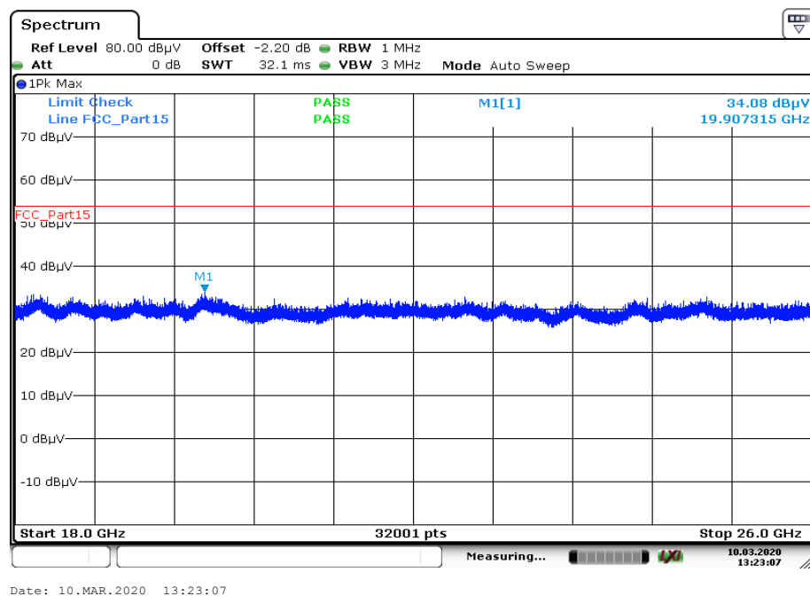
Plot 4: 18 GHz to 26 GHz, TX mode, TX mode on three channels, vertical & horizontal polarization
