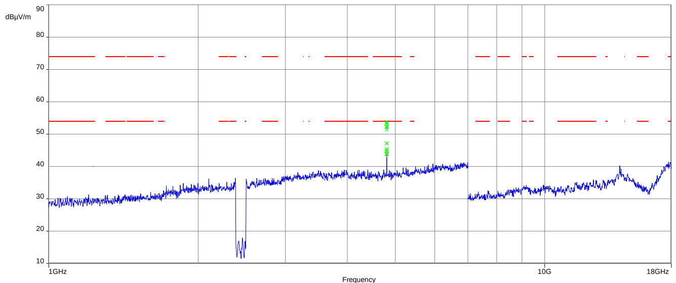
Plot 1: 1 GHz to 18 GHz, TX mode, 2402 MHz, vertical & horizontal polarization
