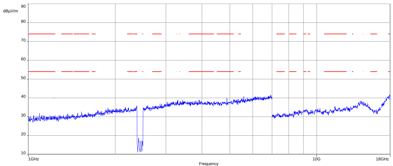
Plot 2: 1 GHz to 18 GHz, TX mode, 2440 MHz, vertical & horizontal polarization
