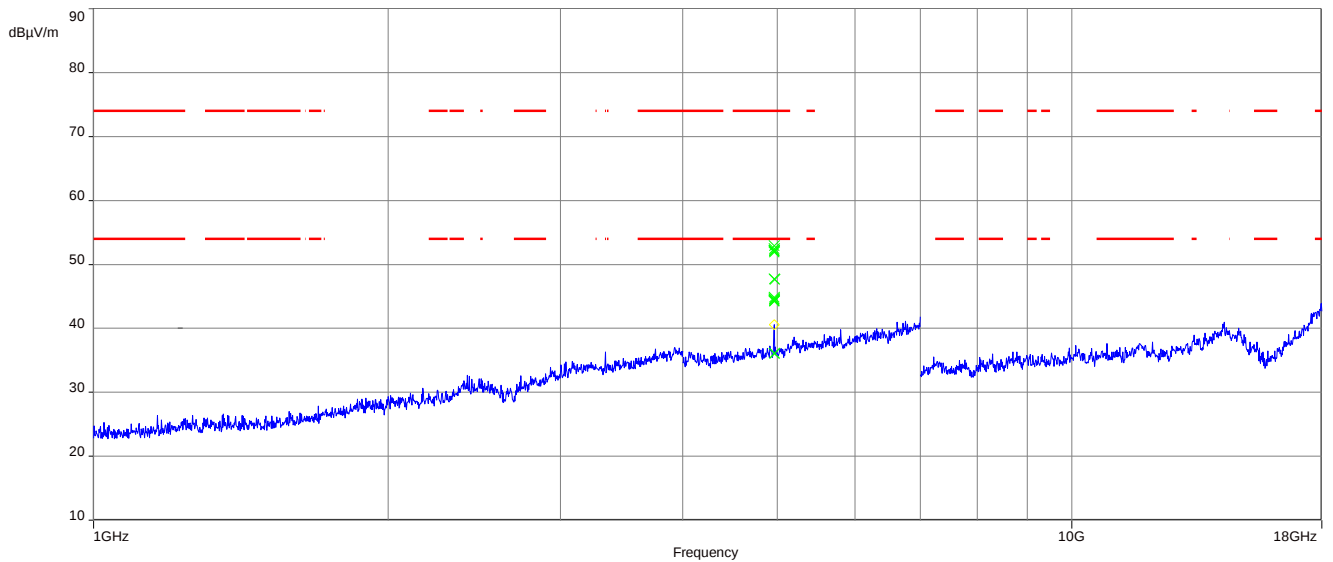
Plot 3: 1 GHz to 18 GHz, TX mode, 2480 MHz, vertical & horizontal polarization, GFSK
