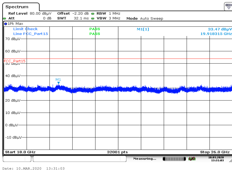
Plot 6: 18 GHz to 26 GHz, TX mode, TX mode on three channels, vertical & horizontal polarization, GFSK
