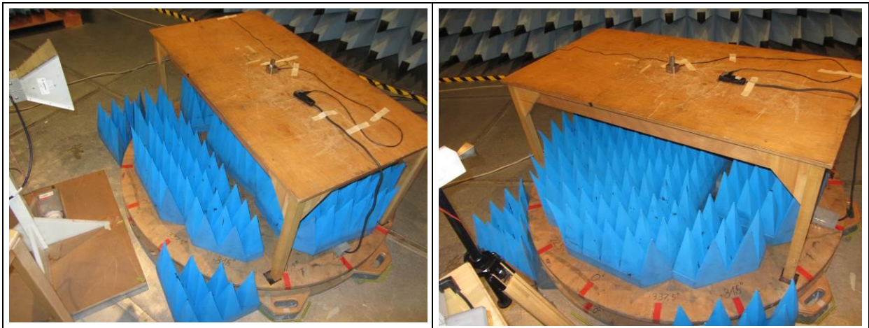
Fig 4 Spurious emissions – 1 GHz- 26.5 GHz
