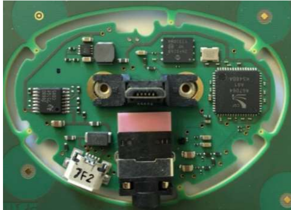
Docking PCB
