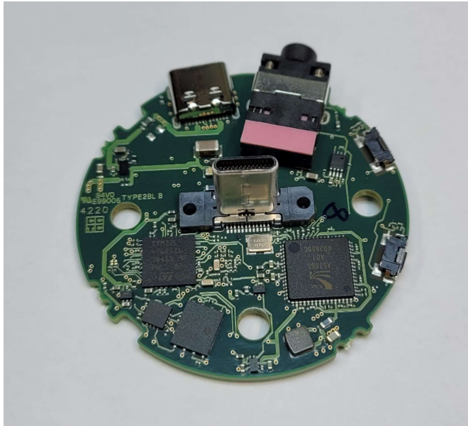
Docking PCB
