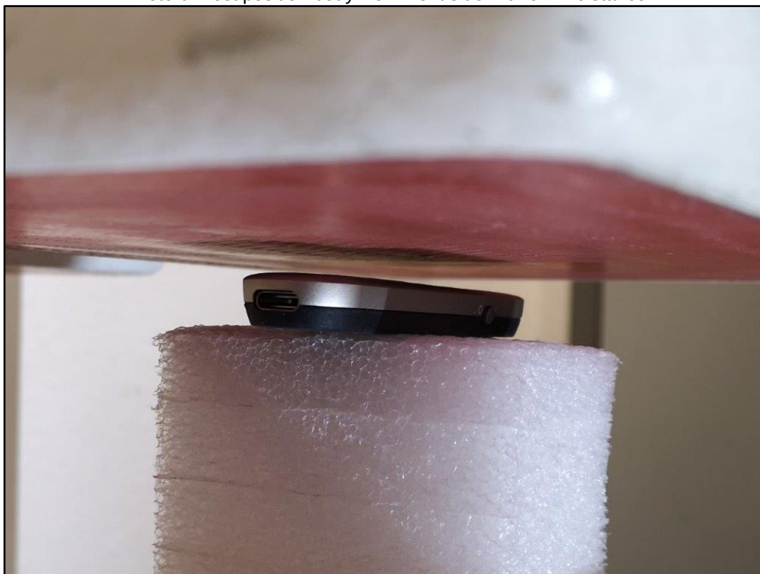
Photo 6: Test position body worn front side with 5mm distance
