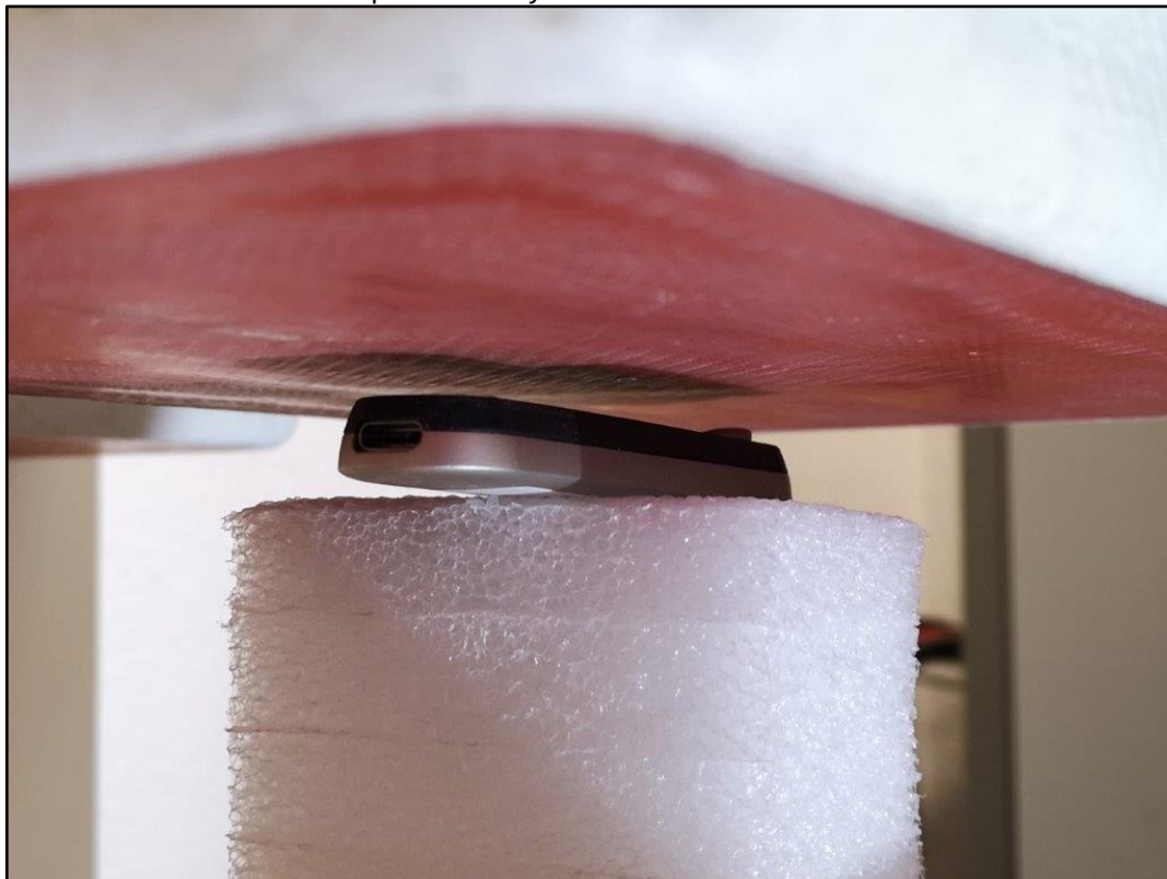
Photo 8: Test position limb front side with 0mm distance
