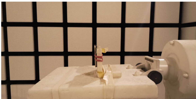
Photo 4: EUT at the anechoic chamber
