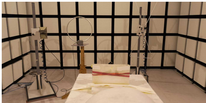
Photo 2: EUT at the anechoic chamber
