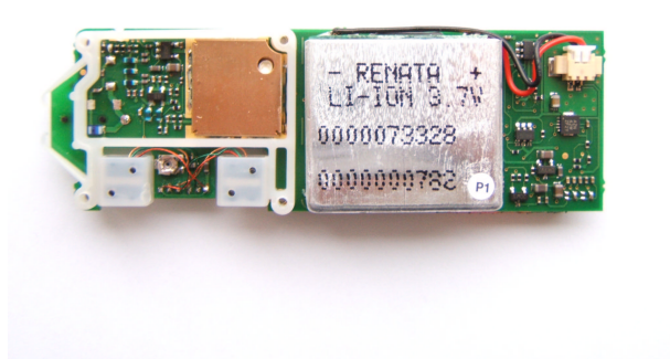
Fig 3: PCB 1 upper side with Li-Ion Battery
