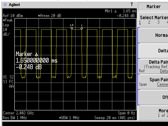
CH 00 2402MHz
