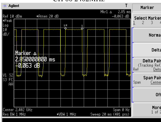
CH 00 2402MHz
