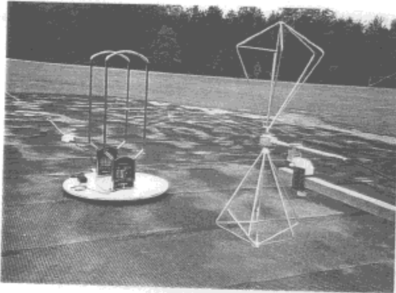
photo 2, measurement setup during the E-field emission measurements at 3 meter
