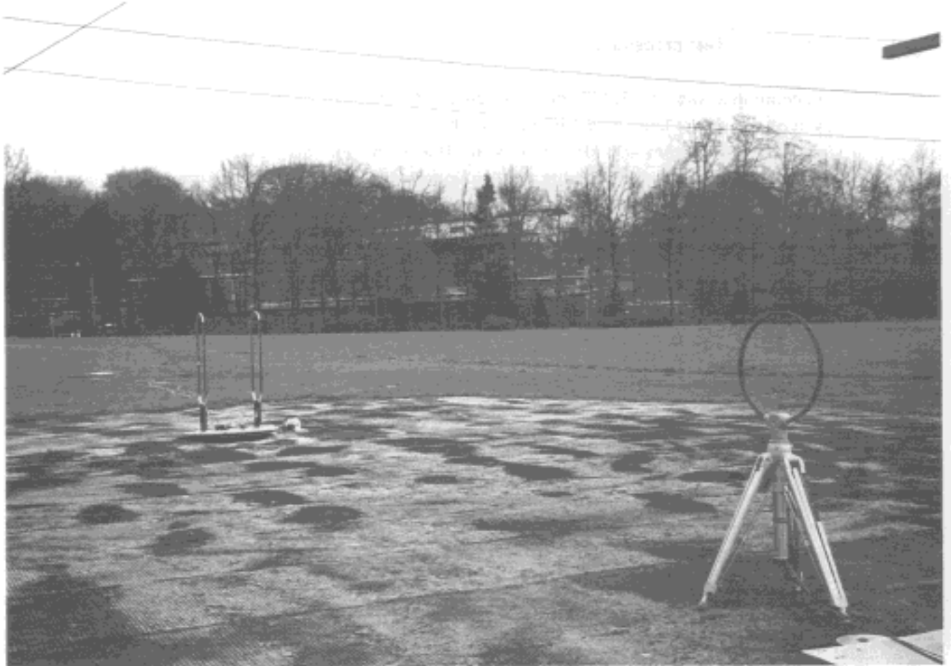
photo 4, measurement setup during the H-field emission measurements at 10 meter
