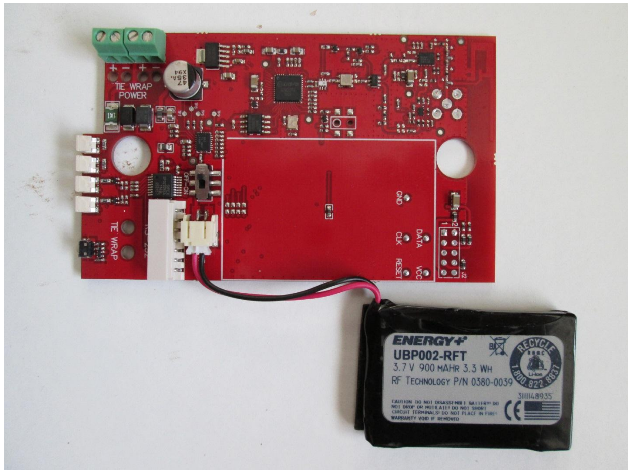
Front Circuit Board Top – with Battery Removed
