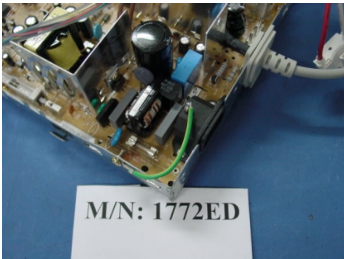
Figure 26 Main Board, Component Side
