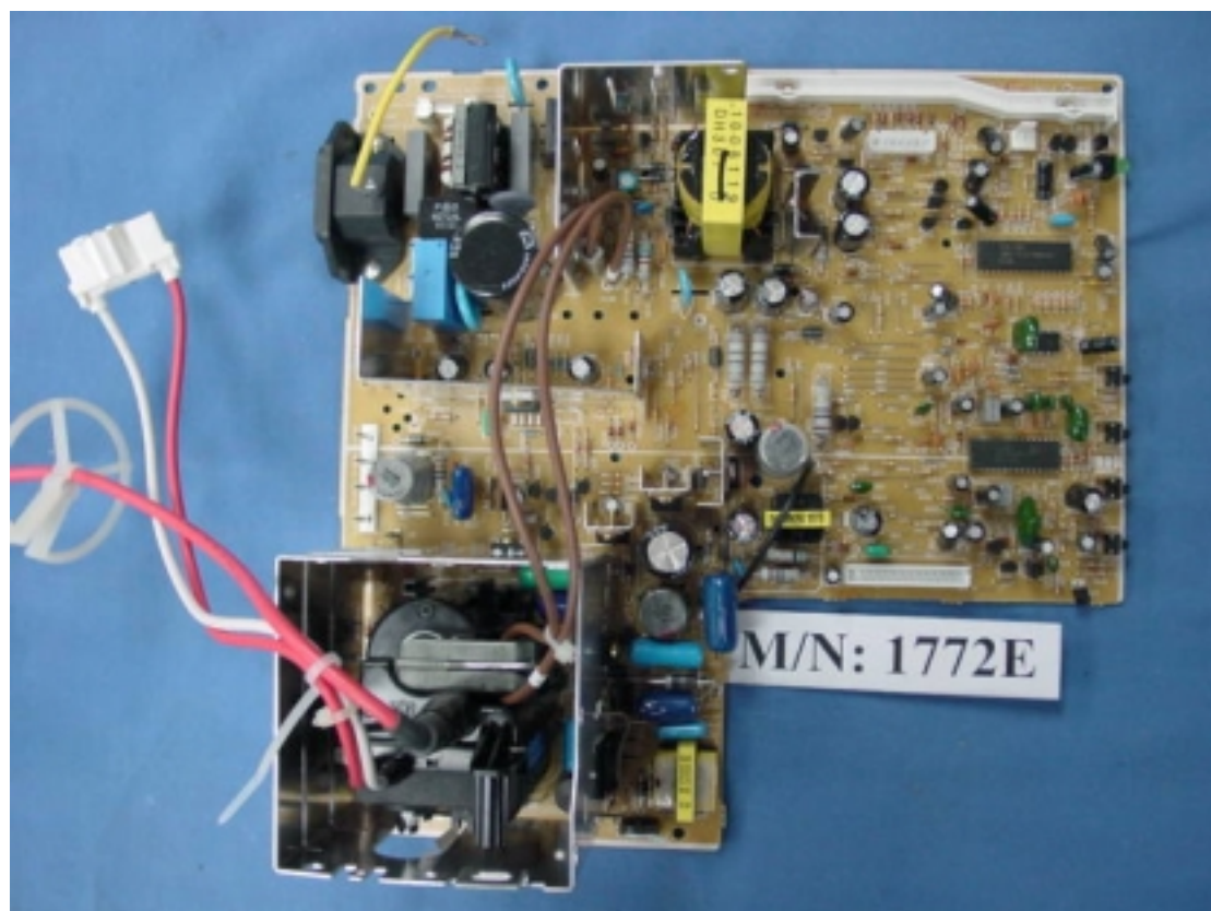
Figure 18 Main Board, Component Side
