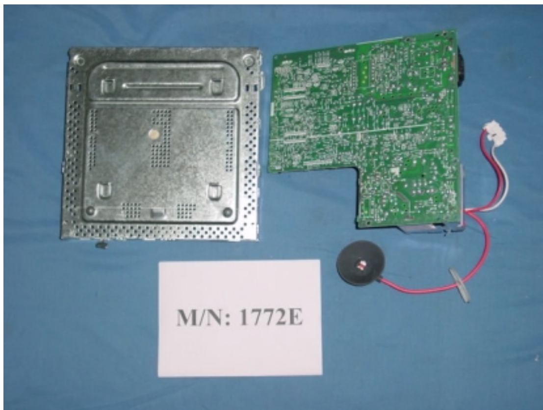
Figure 14 Main Board, Component Side
