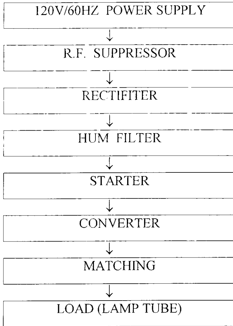
BLOCK DIAGRAM OF 120V DIRECT RECTIFYING LAMP SERIES
