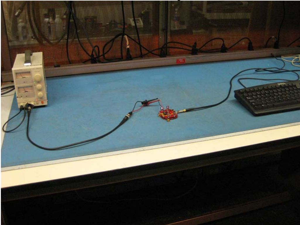
Conducted Testing #2
