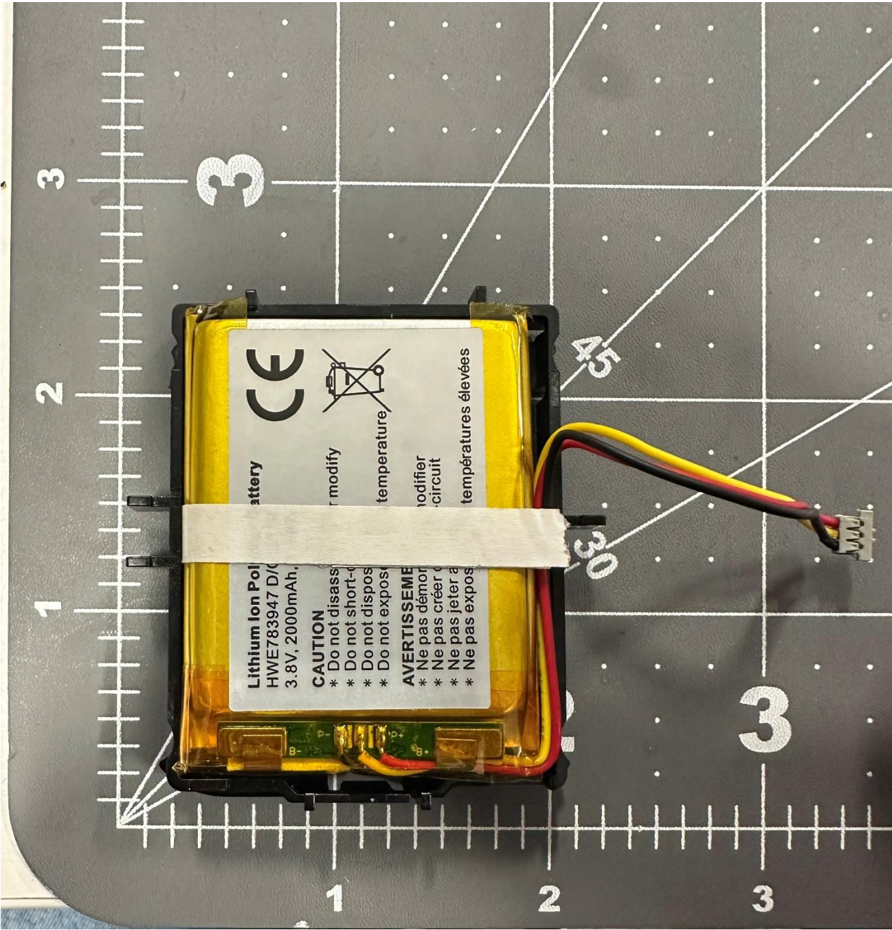
Battery / battery carrier removed from front housing
