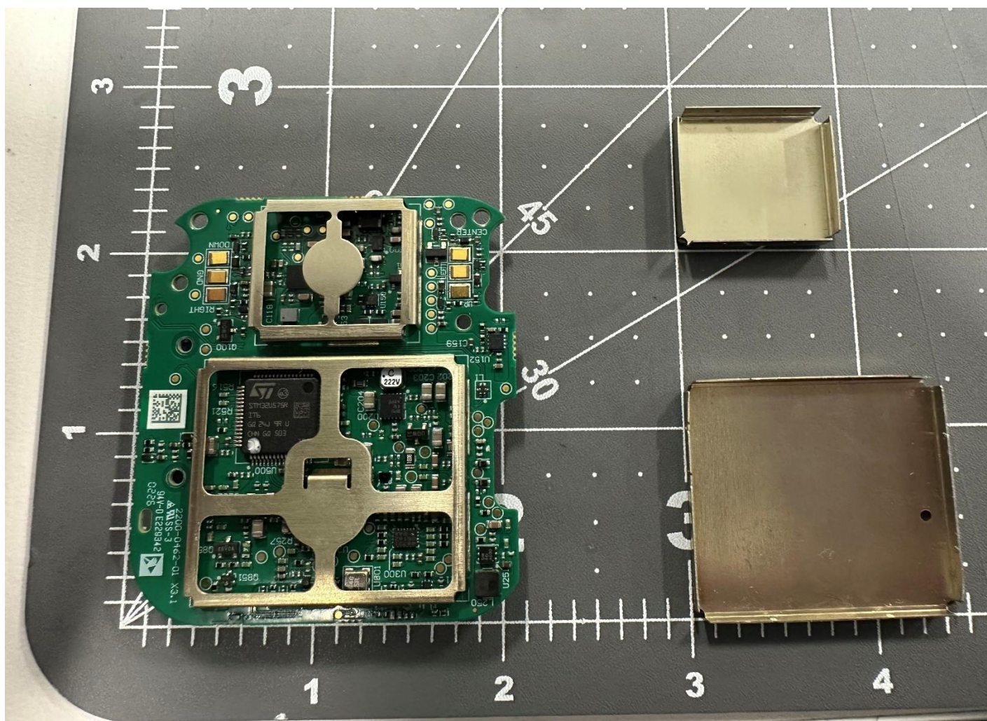
Top of PCBA w/ shields removed
