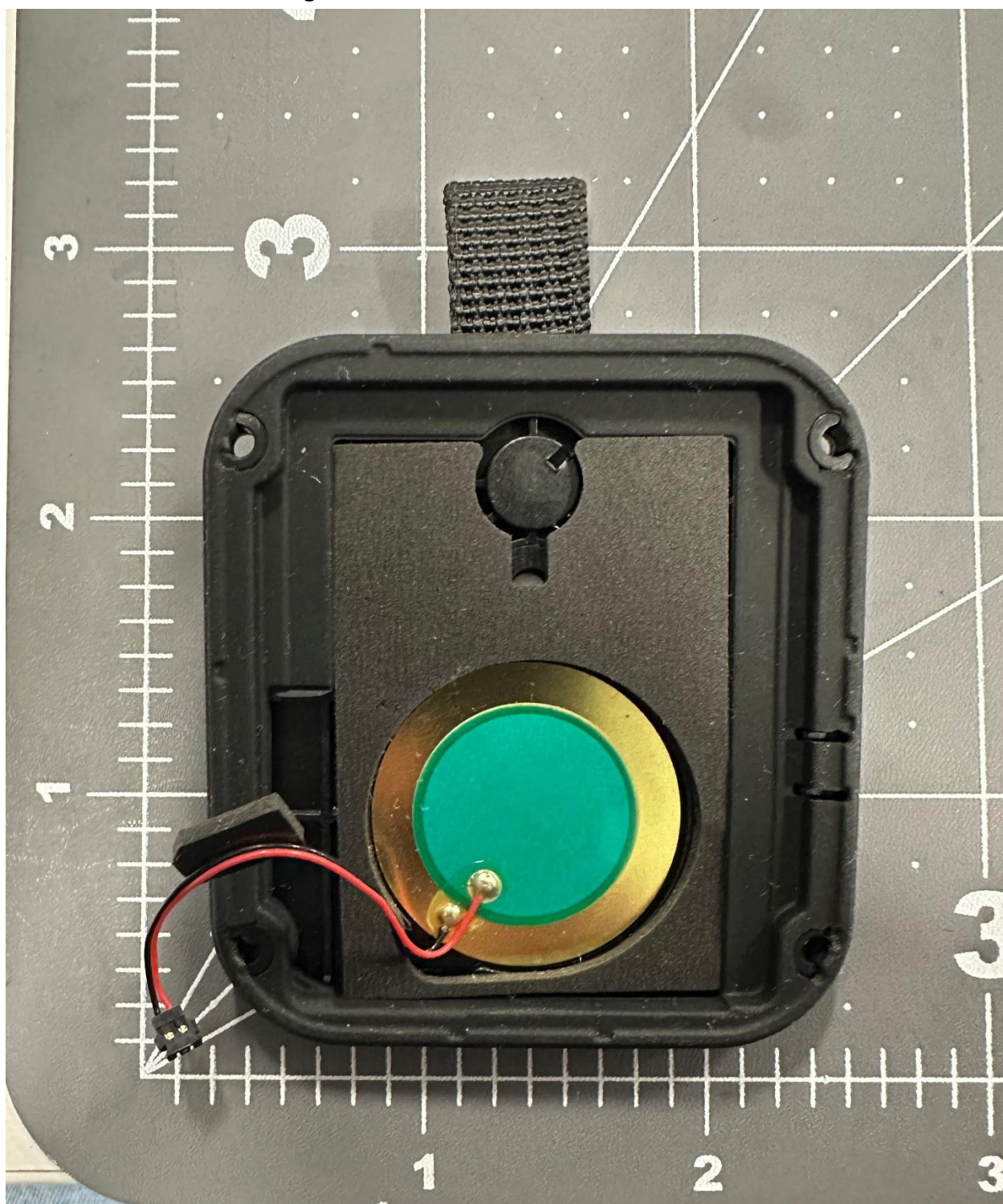
Inside View of Back Housing
