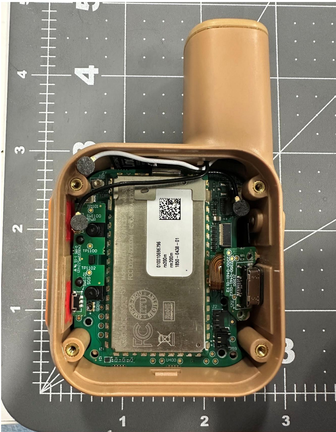
Inside View of Front Housing – View of Bottom of PCBA after battery and battery carrier removal
