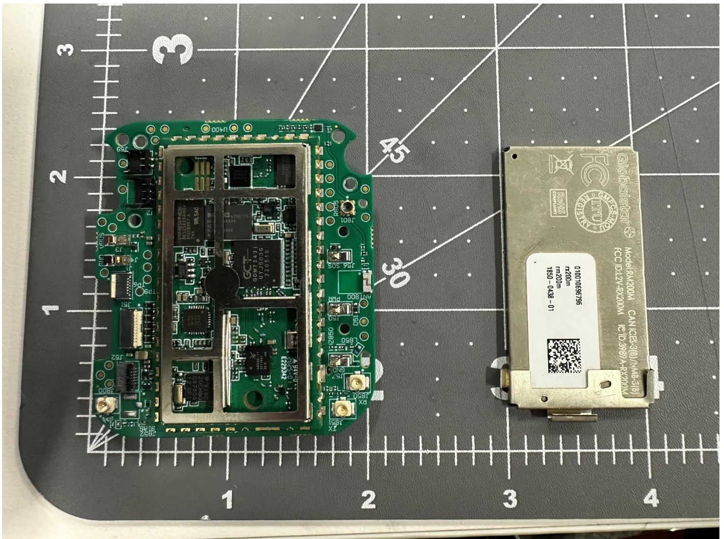
Bottom of PCBA w/ top shield removed
