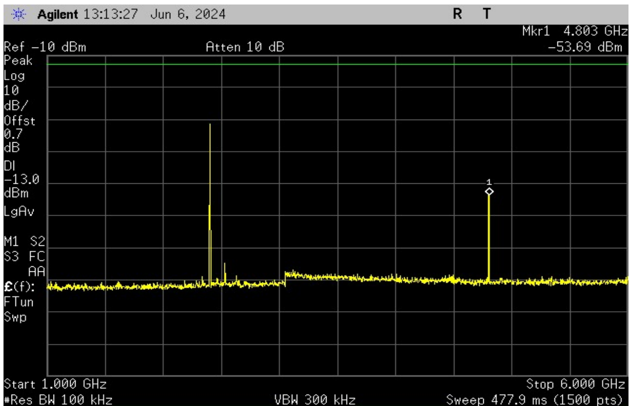
Plot 10 – Low Band – 1GHz to 6GHz
