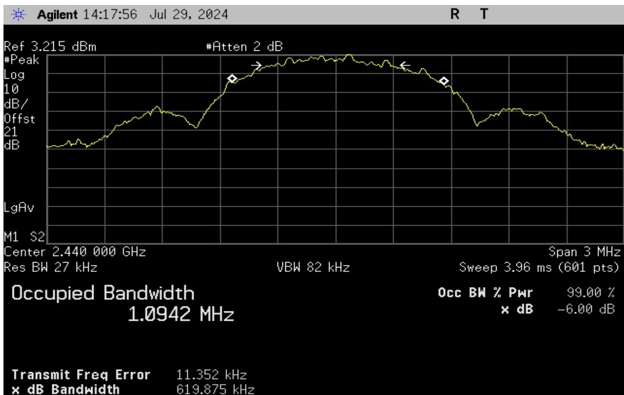
Plot 4 – Middle Channel – 6dB BW
