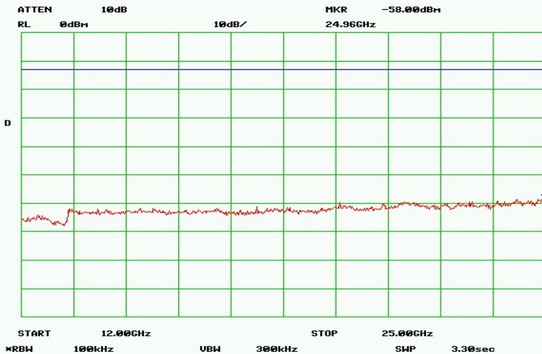
Plot 20 – High Band – 12GHz to 25GHz
