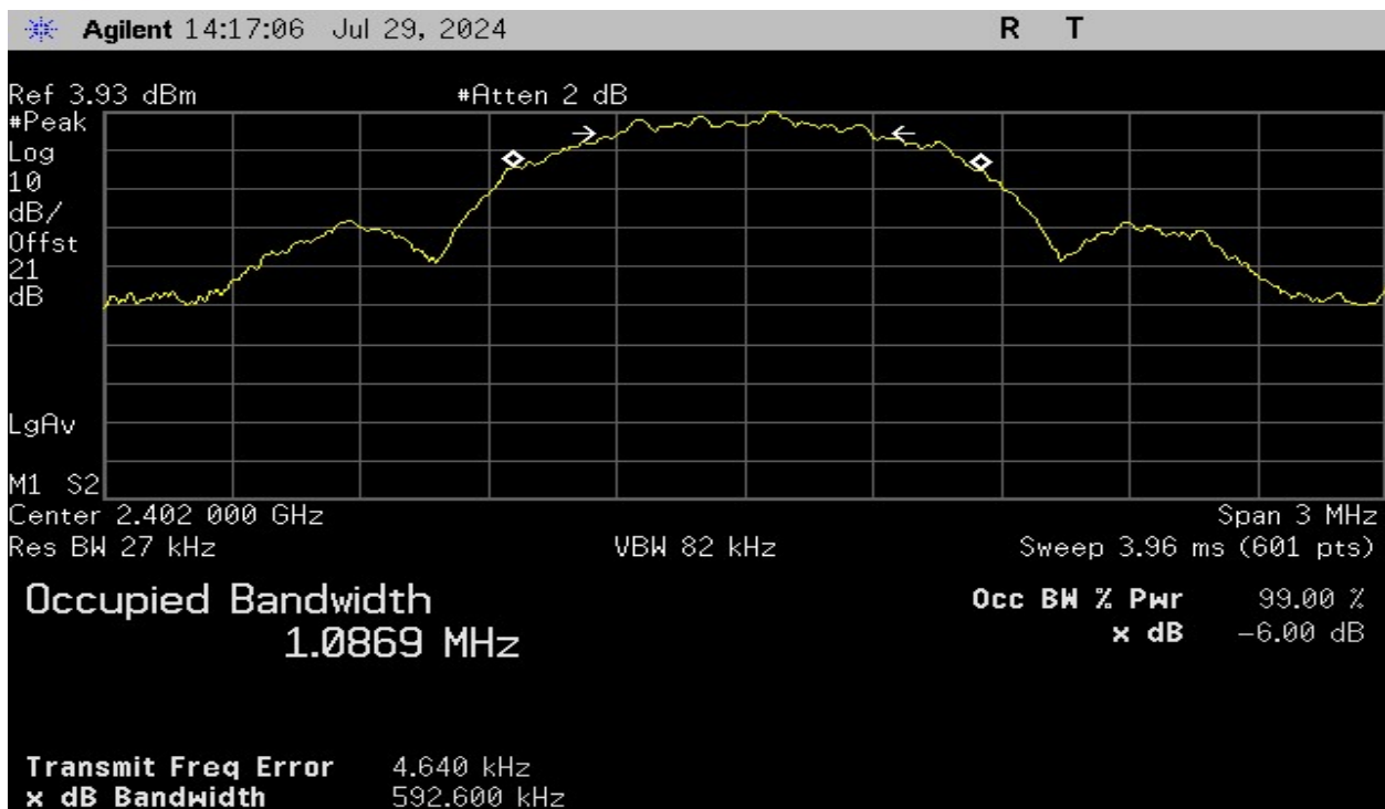
Plot 3 – Lowest Channel – 6dB BW
