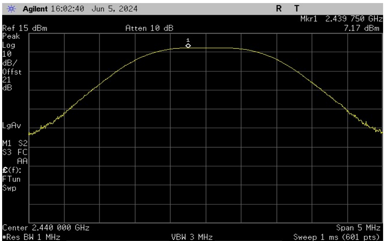
Plot 7 – Output Power – Middle Channel
