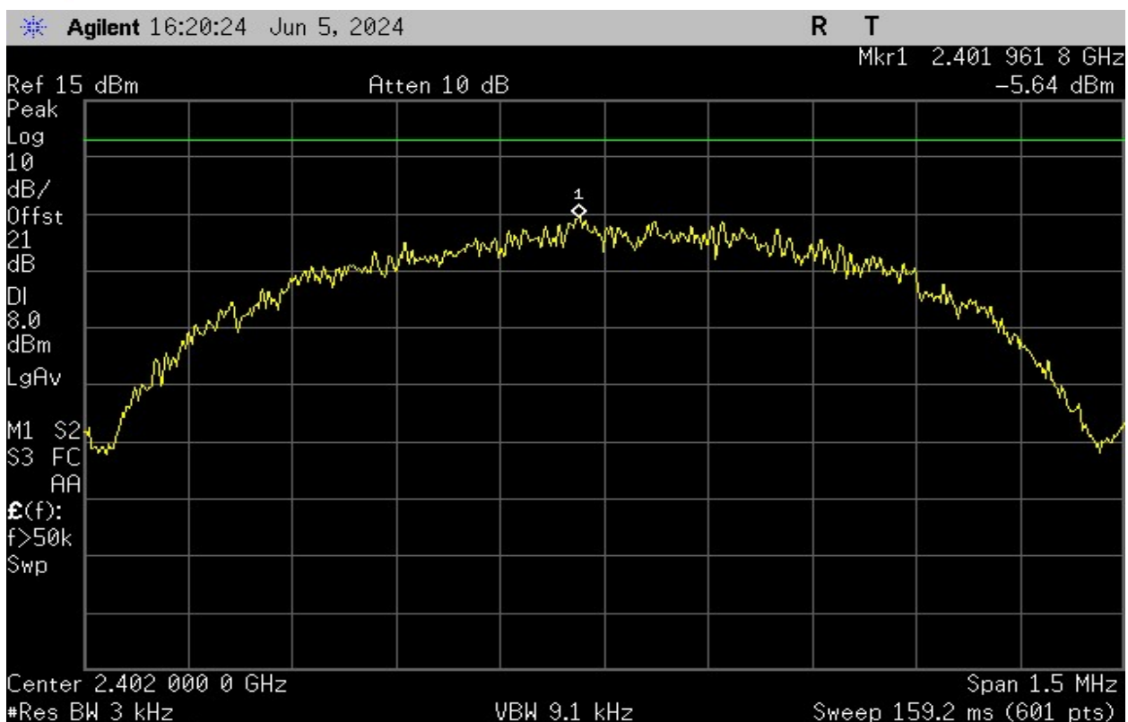
Plot 23 – Power Spectral Density – Lowest Channel
