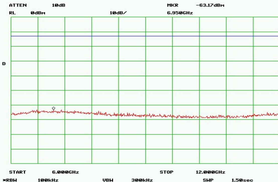
Plot 11 – Low Band – 6GHz to 12GHz
