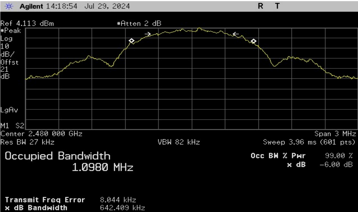
Plot 5 – Highest Channel – 6dB BW
