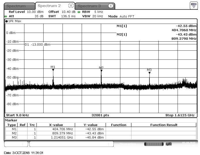
Figure 7.3.1.2-8: 9 kHz – 1.6125 GHz – High Channel
