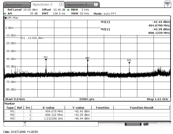
Figure 7.3.1.2-6: 9 kHz – 1.61 GHz – Middle Channel
